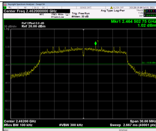
802.11n(HT20),2462MHz,Ant0,Plot 1,Reference Level
