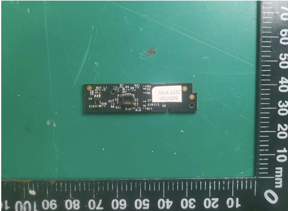
Radar PCB
