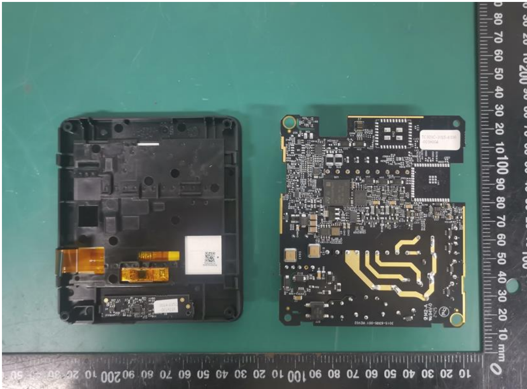
Radar PCB
