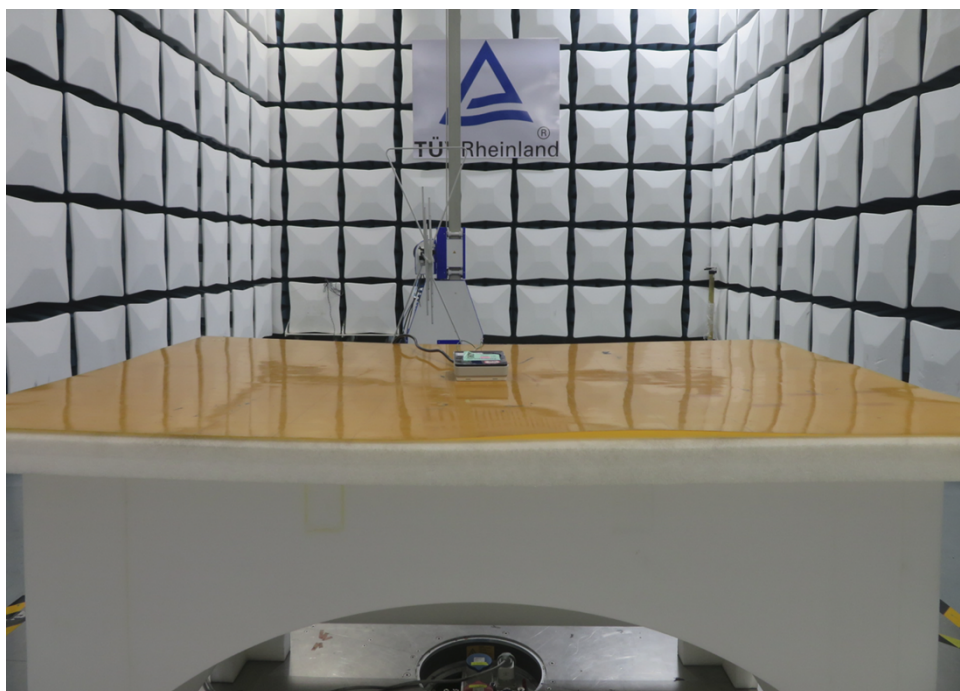
Photograph 1: Set-up photo for Radiated Emission, Below 1GHz
