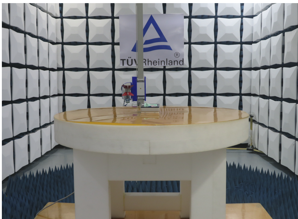
Photograph 2: Set-up photo for Radiated Emission, Above 1GHz
