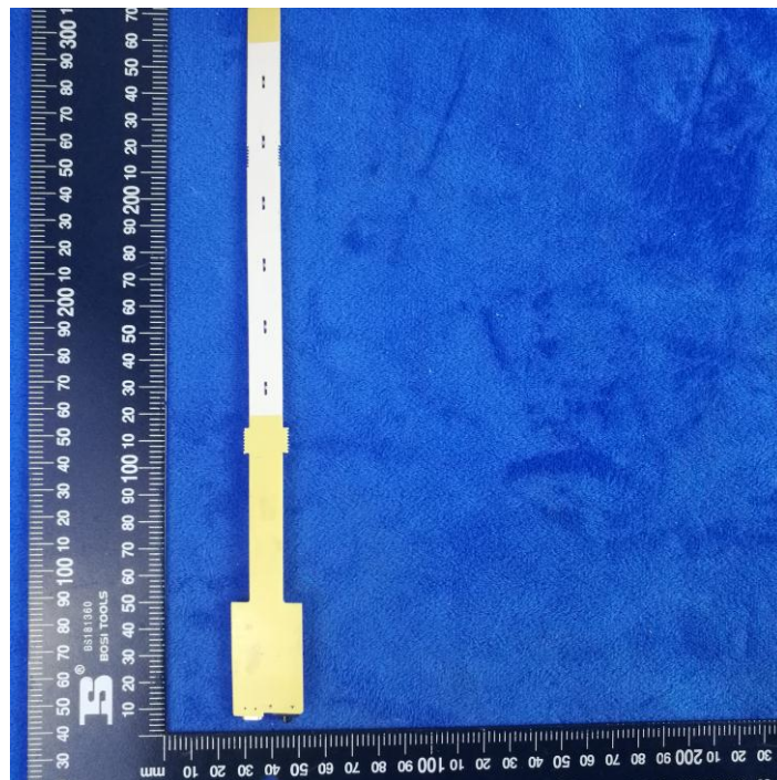
PCB – Rear View
