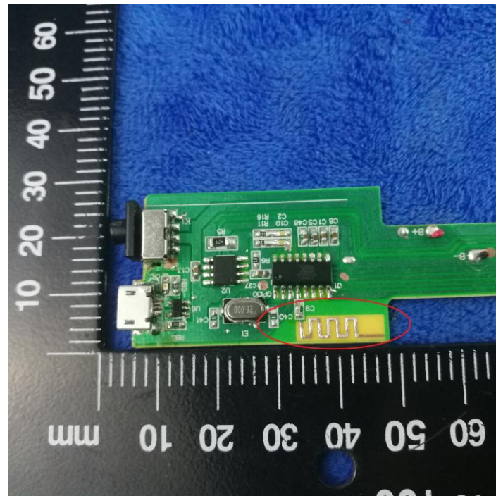
Antenna View
