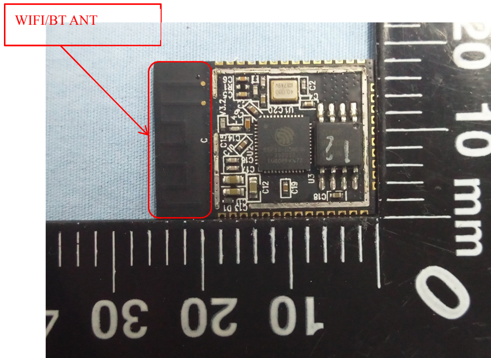
Solder Board-Component View 7
