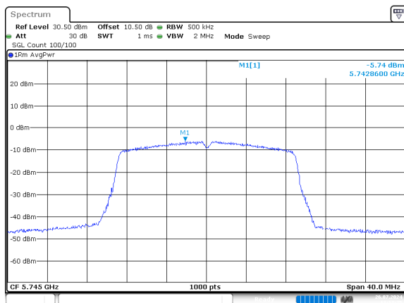
n20_5745MHz_Chain 0
