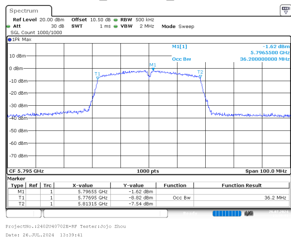
n40_5795MHz_Chain 0
