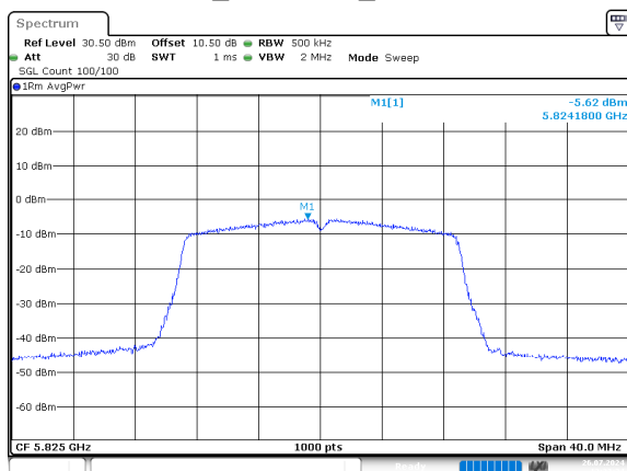
n20_5825MHz_Chain 0
