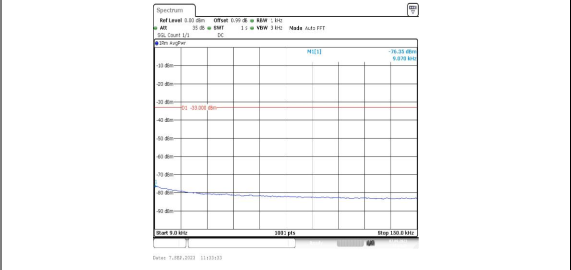
Band5-4132-4-0.009~0.15MHz-PASS
