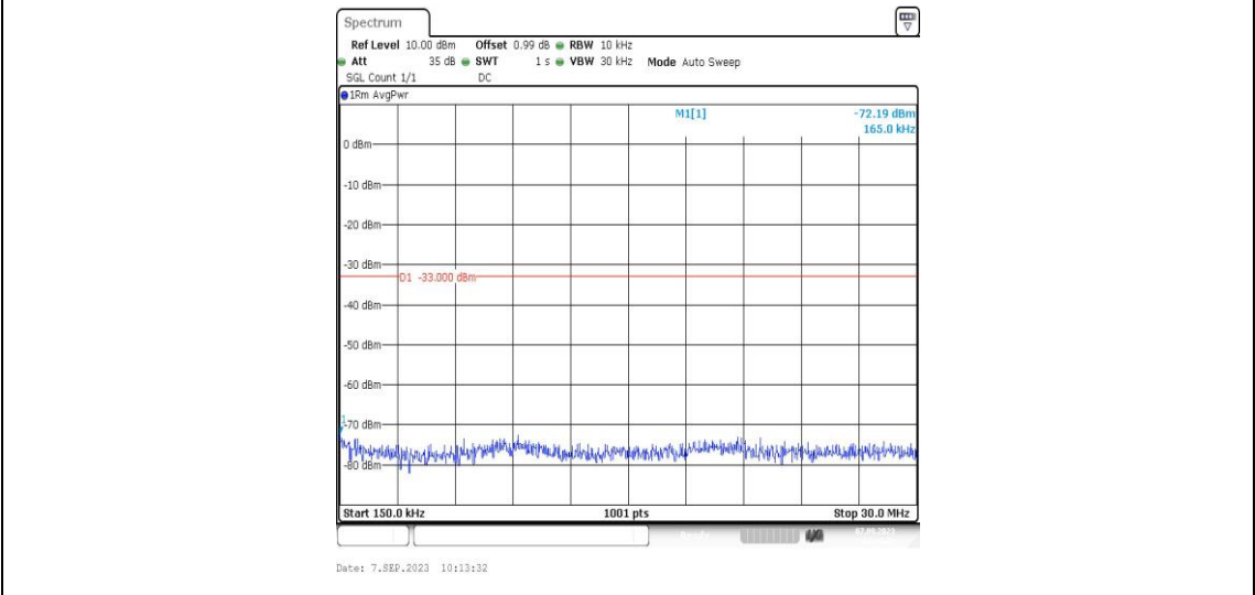
Band2-9538-4-0.15~30MHz-PASS
