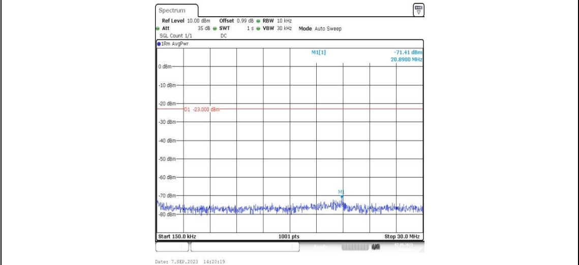
Band5-4233-2-0.15~30MHz-PASS
