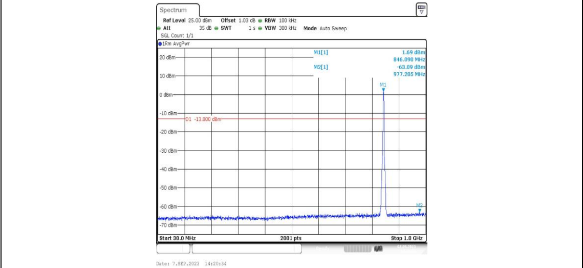
Band5-4233-2-30~1000MHz-PASS
