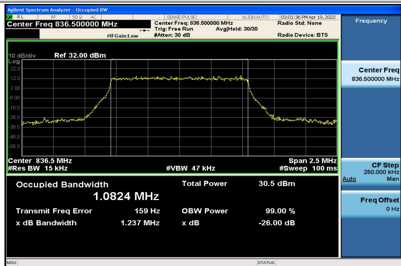
Band5-1.4MHz-QPSK-20525-6RB#0-1.0824
