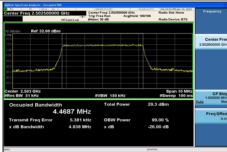
Band7-5MHz-16QAM-20775-25RB#0-4.4687
