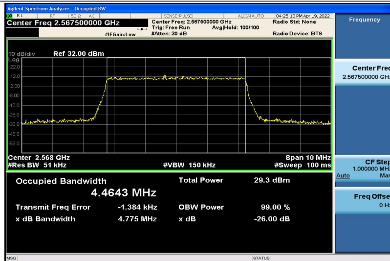
Band7-5MHz-16QAM-21425-25RB#0-4.4643
