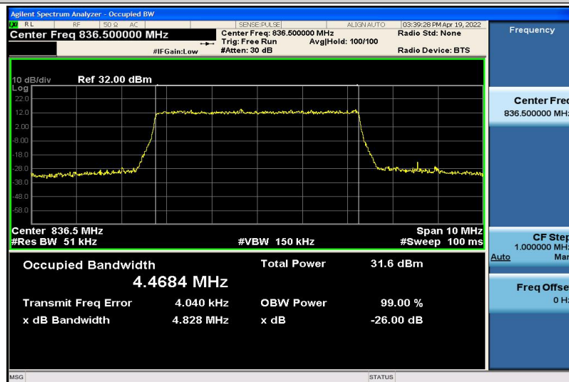
Band5-5MHz-QPSK-20525-25RB#0-4.4684
