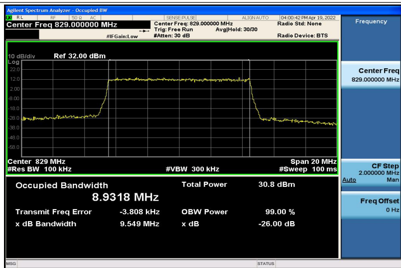
Band5-10MHz-16QAM-20450-50RB#0-8.9318
