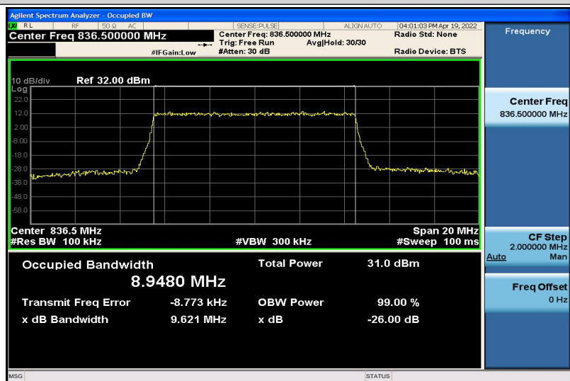
Band5-10MHz-16QAM-20525-50RB#0-8.9480
