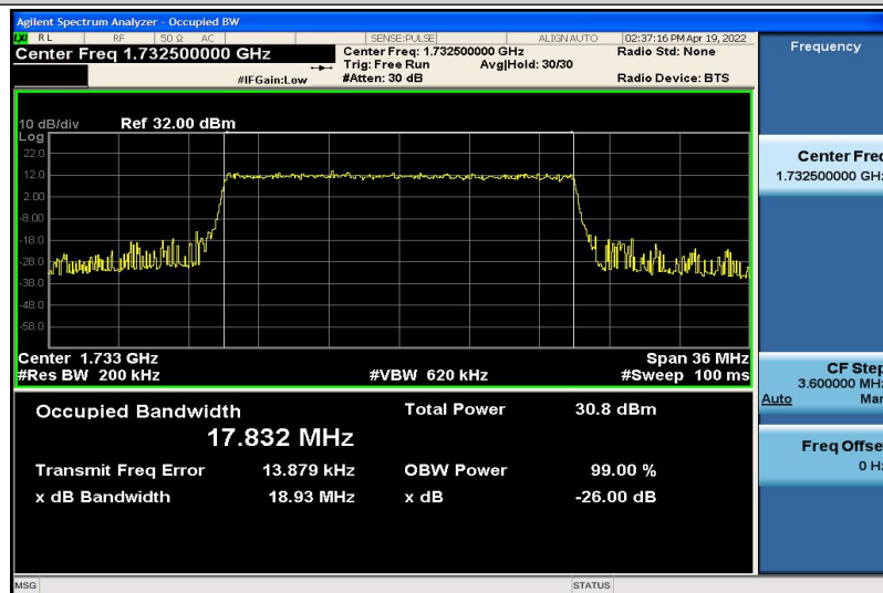
Band4-20MHz-QPSK-20175-100RB#0-17.832
