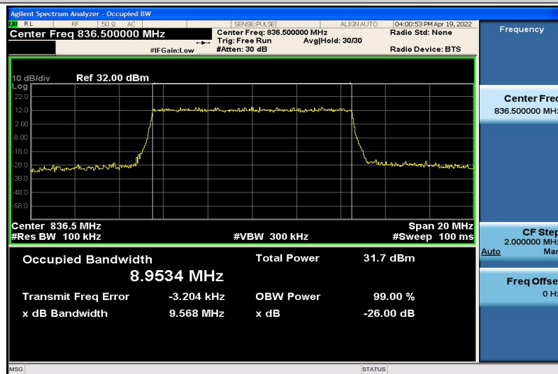
Band5-10MHz-QPSK-20525-50RB#0-8.9534
