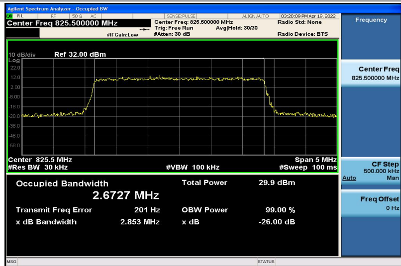
Band5-3MHz-16QAM-20415-15RB#0-2.6727
