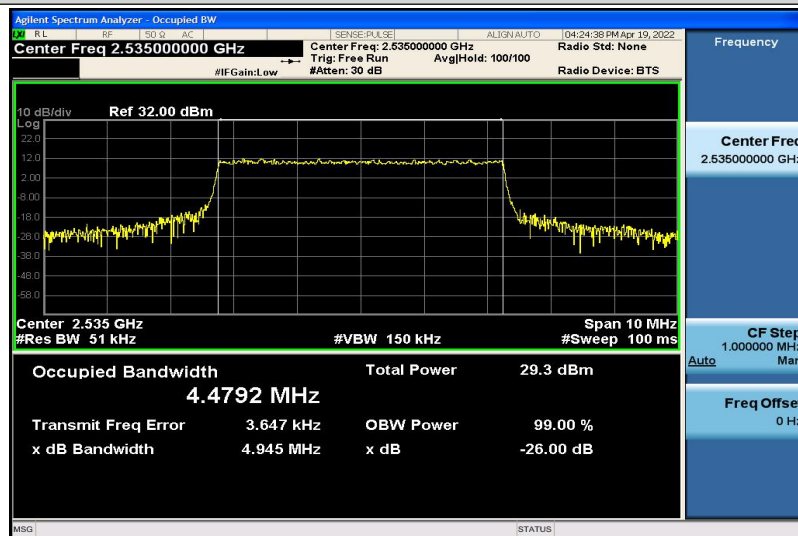
Band7-5MHz-16QAM-21100-25RB#0-4.4792
