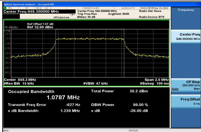
Band5-1.4MHz-QPSK-20643-6RB#0-1.0787
