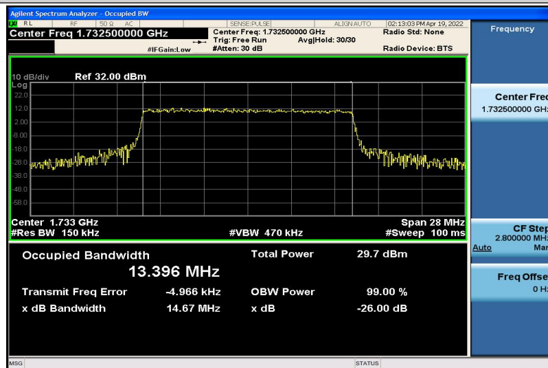
Band4-15MHz-QPSK-20175-75RB#0-13.396
