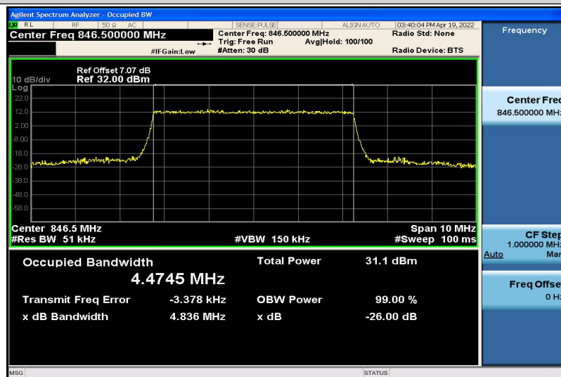
Band5-5MHz-QPSK-20625-25RB#0-4.4745
