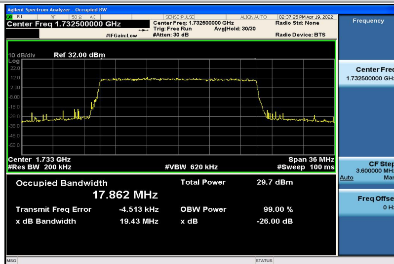
Band4-20MHz-16QAM-20175-100RB#0-17.862
