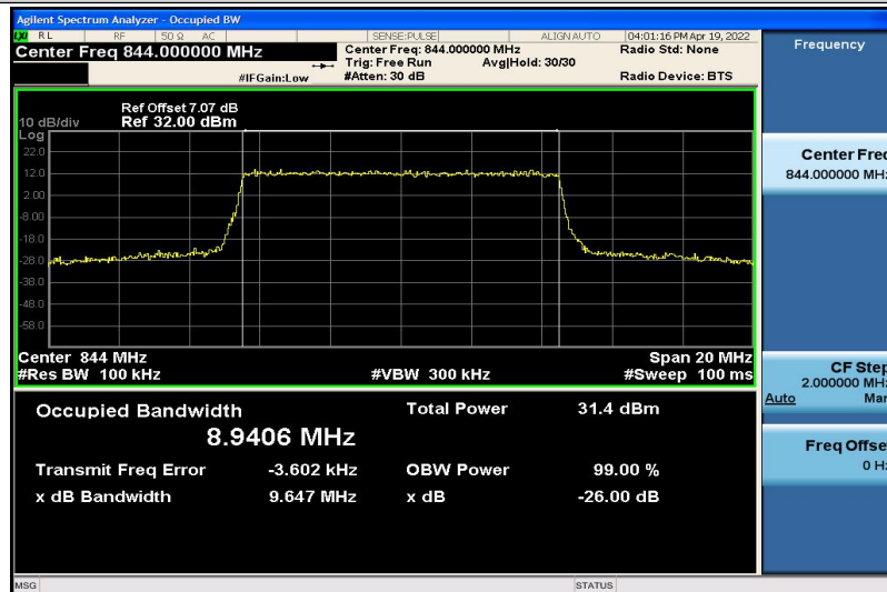
Band5-10MHz-QPSK-20600-50RB#0-8.9406
