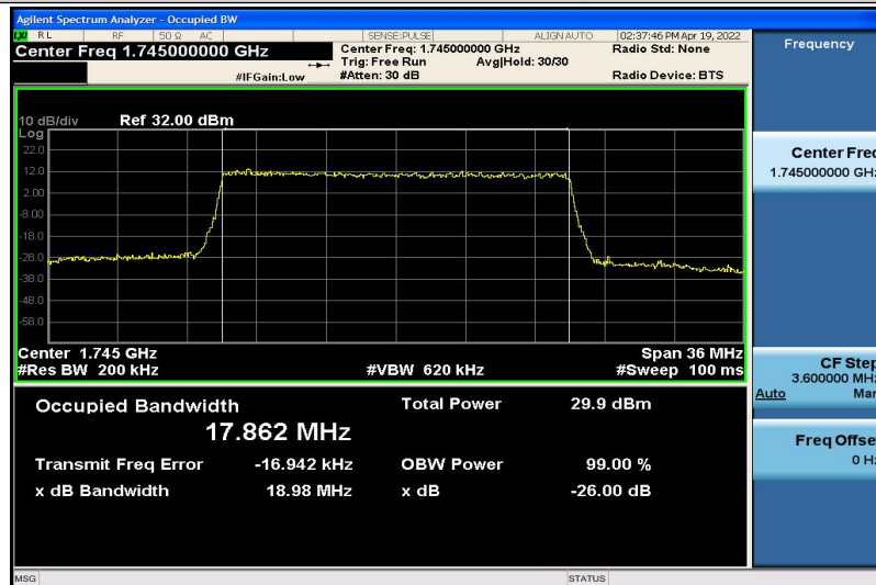
Band4-20MHz-16QAM-20300-100RB#0-17.862
