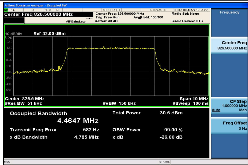
Band5-5MHz-16QAM-20425-25RB#0-4.4647
