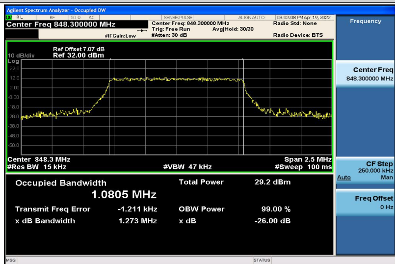
Band5-1.4MHz-16QAM-20643-6RB#0-1.0805
