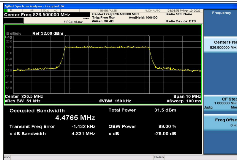
Band5-5MHz-QPSK-20425-25RB#0-4.4765
