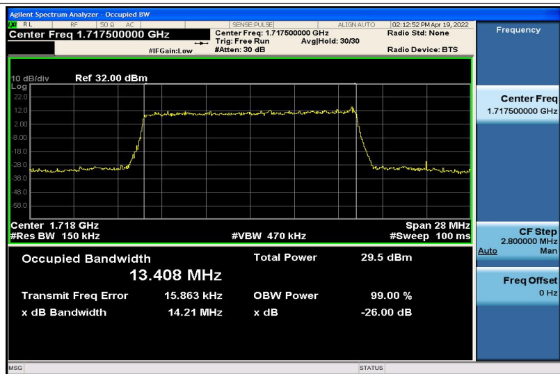
Band4-15MHz-16QAM-20025-75RB#0-13.408
