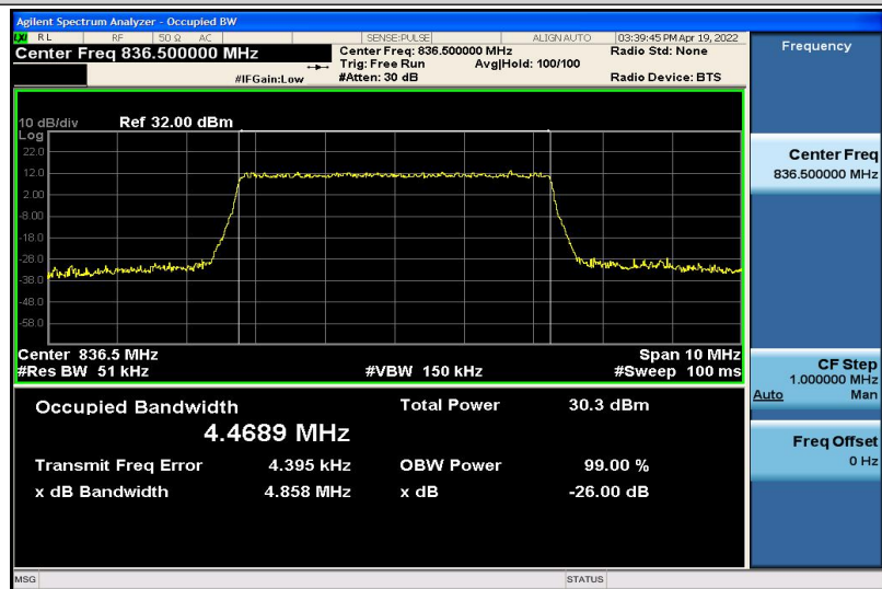
Band5-5MHz-16QAM-20525-25RB#0-4.4689
