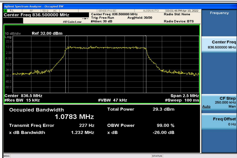
Band5-1.4MHz-16QAM-20525-6RB#0-1.0783
