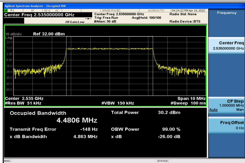
Band7-5MHz-QPSK-21100-25RB#0-4.4806
