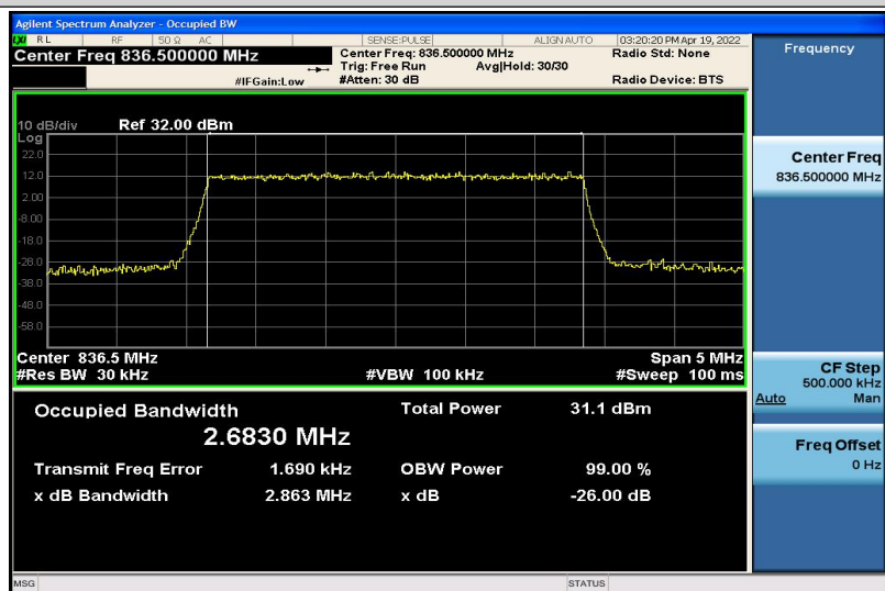
Band5-3MHz-QPSK-20525-15RB#0-2.6830
