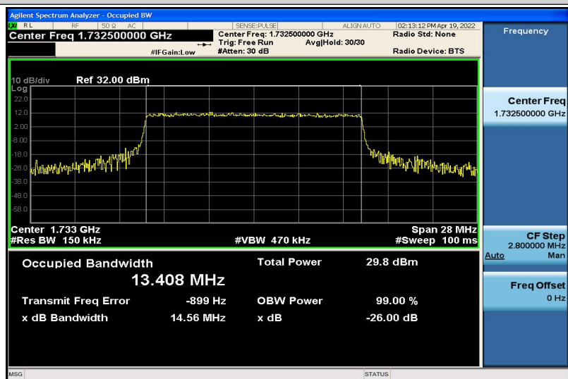
Band4-15MHz-16QAM-20175-75RB#0-13.408
