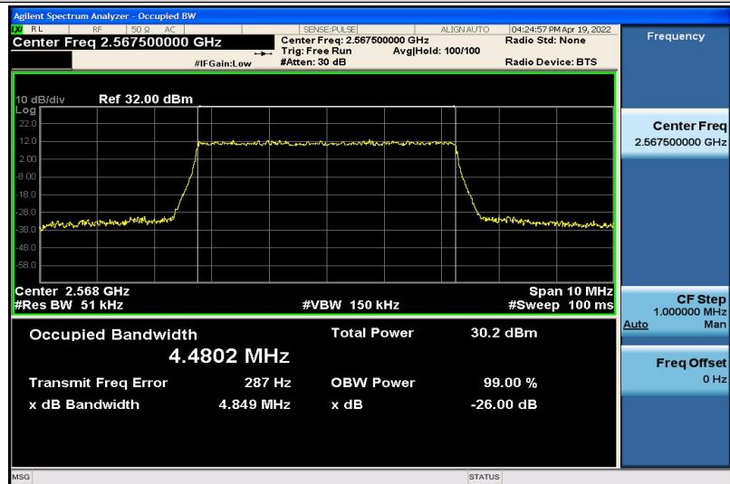
Band7-5MHz-QPSK-21425-25RB#0-4.4802
