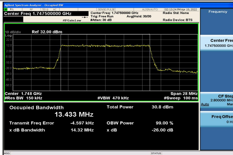
Band4-15MHz-QPSK-20325-75RB#0-13.433
