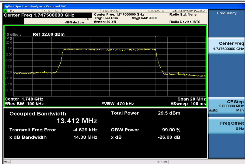
Band4-15MHz-16QAM-20325-75RB#0-13.412
