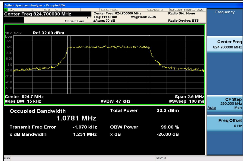
Band5-1.4MHz-QPSK-20407-6RB#0-1.0781
