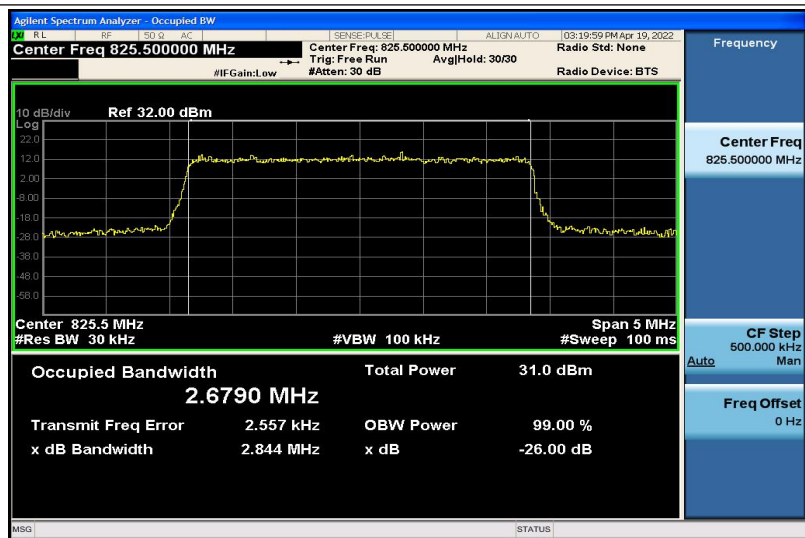
Band5-3MHz-QPSK-20415-15RB#0-2.6790
