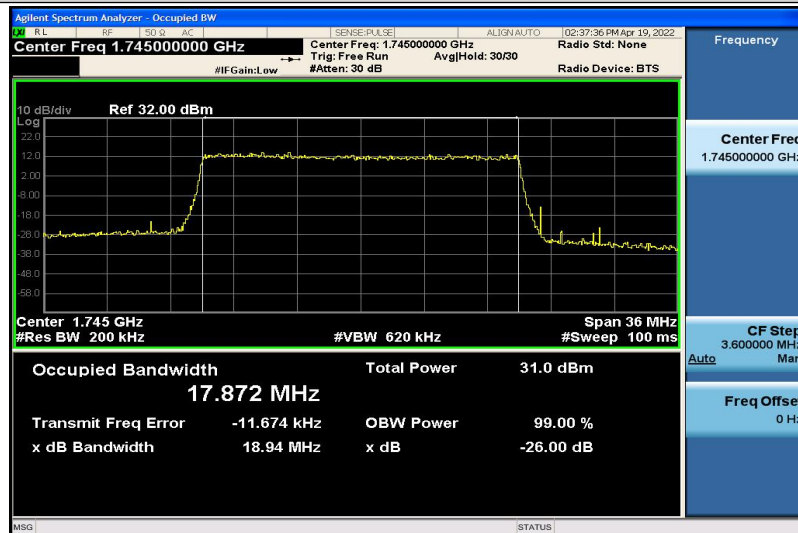
Band4-20MHz-QPSK-20300-100RB#0-17.872
