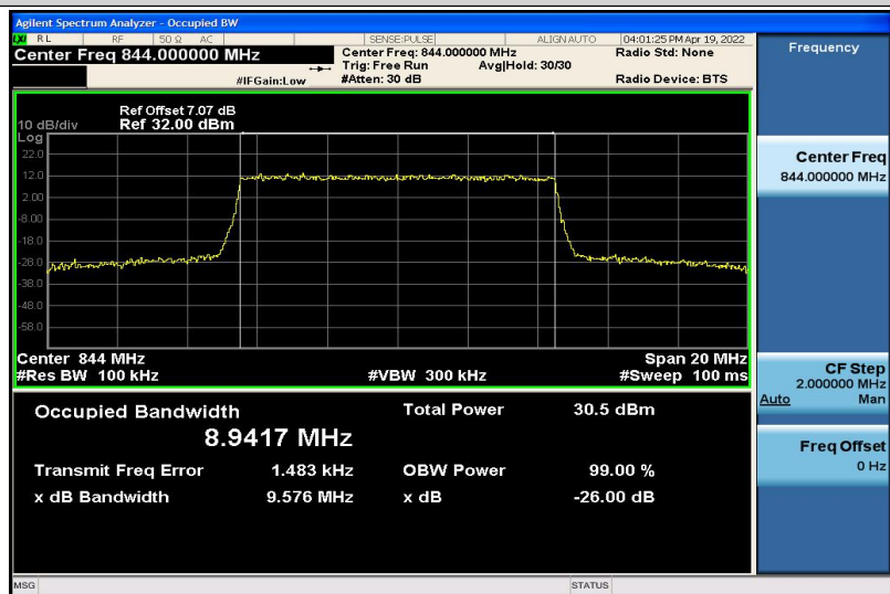
Band5-10MHz-16QAM-20600-50RB#0-8.9417
