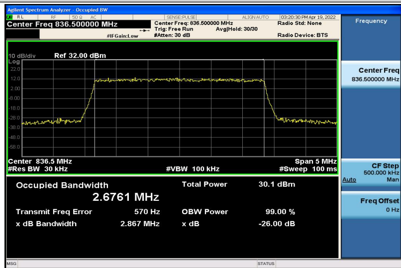
Band5-3MHz-16QAM-20525-15RB#0-2.6761
