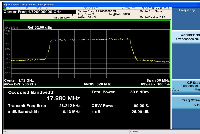
Band4-20MHz-QPSK-20050-100RB#0-17.880
