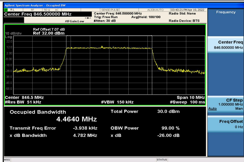
Band5-5MHz-16QAM-20625-25RB#0-4.4640
