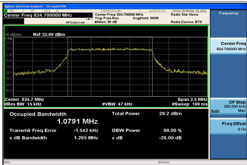
Band5-1.4MHz-16QAM-20407-6RB#0-1.0791
