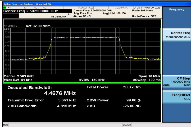
Band7-5MHz-QPSK-20775-25RB#0-4.4676
