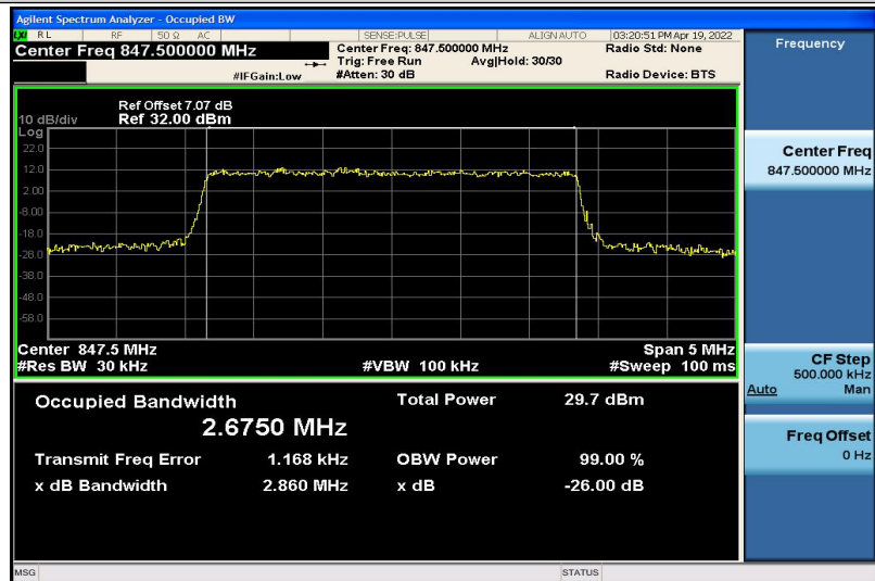
Band5-3MHz-16QAM-20635-15RB#0-2.6750
