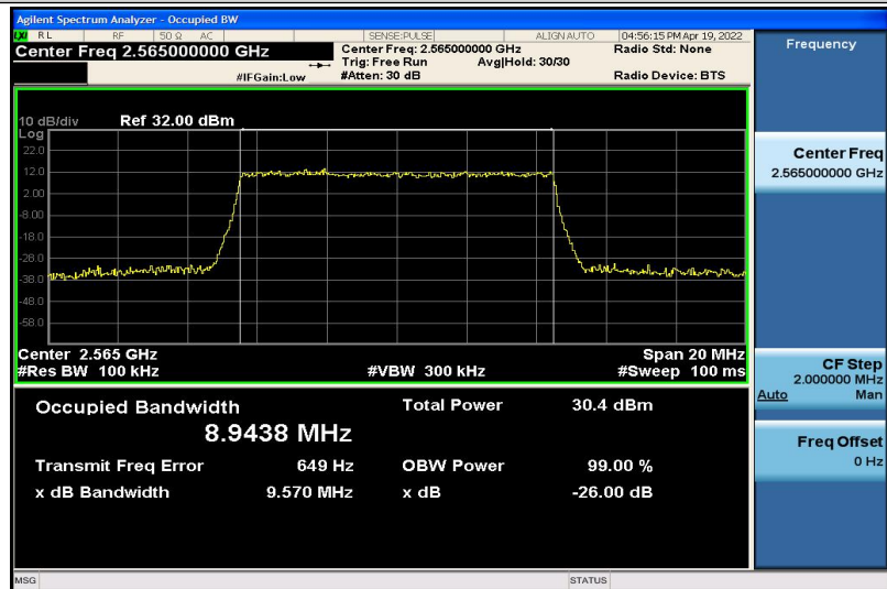
Band7-10MHz-QPSK-21400-50RB#0-8.9438
