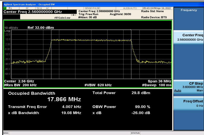
Band7-20MHz-QPSK-21350-100RB#0-17.866
