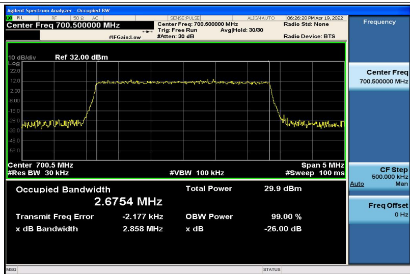
Band12-3MHz-16QAM-23025-15RB#0-2.6754
