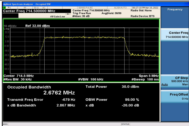
Band12-3MHz-16QAM-23165-15RB#0-2.6762
