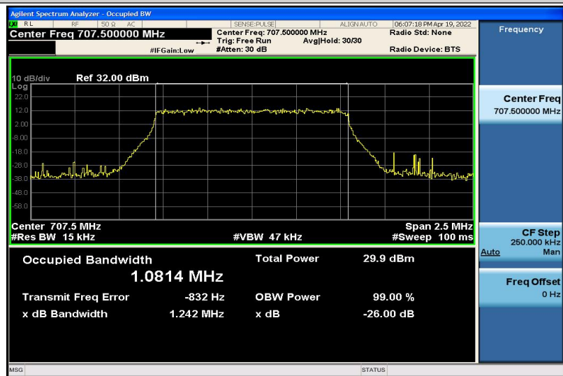
Band12-1.4MHz-QPSK-23095-6RB#0-1.0814
