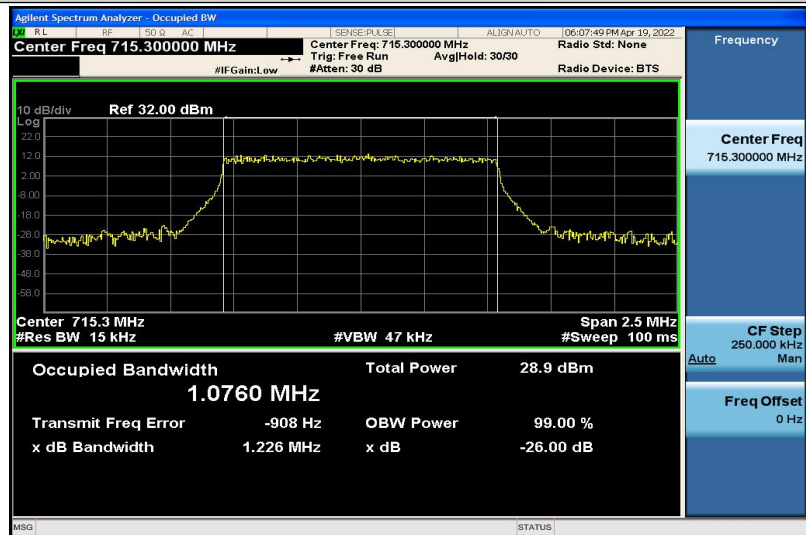
Band12-1.4MHz-16QAM-23173-6RB#0-1.0760
