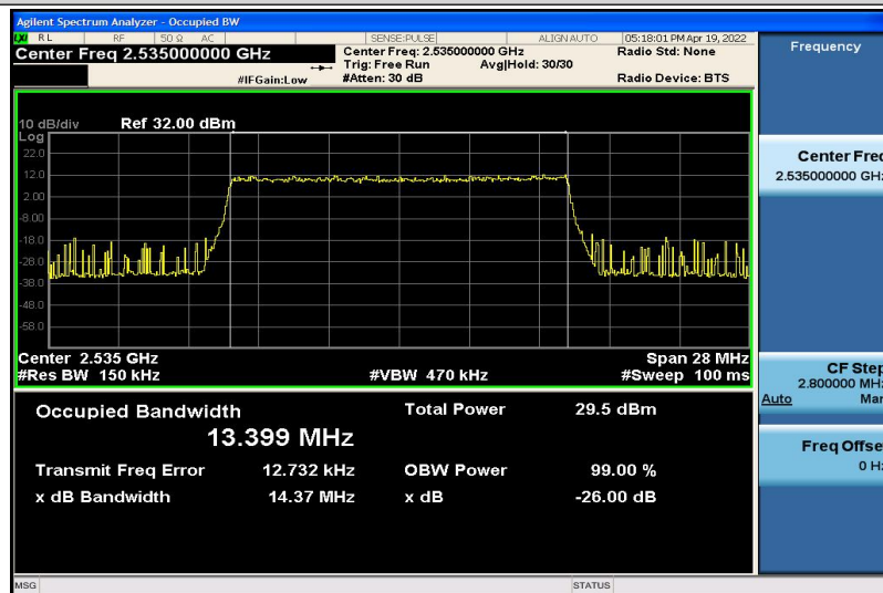
Band7-15MHz-16QAM-21100-75RB#0-13.399
