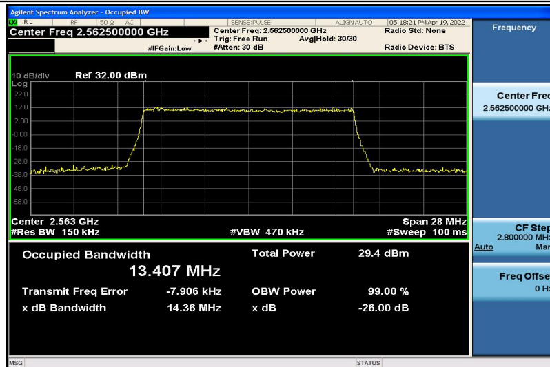
Band7-15MHz-16QAM-21375-75RB#0-13.407
