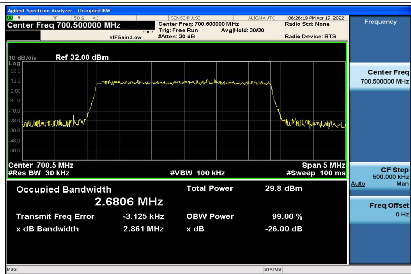
Band12-3MHz-QPSK-23025-15RB#0-2.6806
