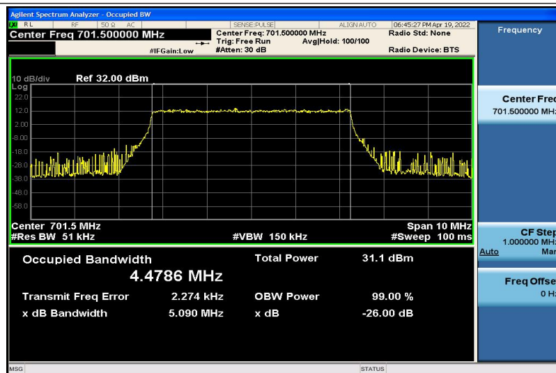
Band12-5MHz-QPSK-23035-25RB#0-4.4786
