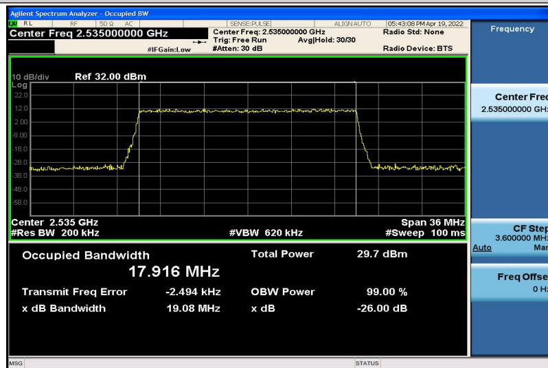
Band7-20MHz-16QAM-21100-100RB#0-17.916
