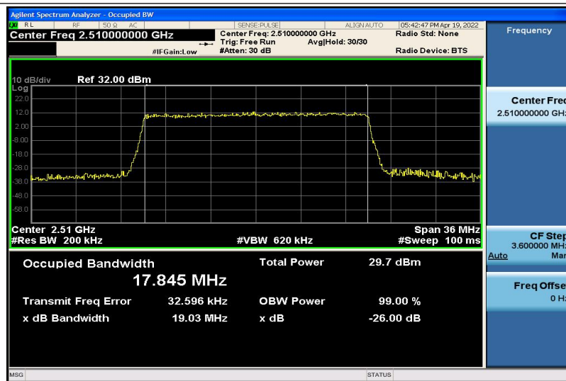
Band7-20MHz-16QAM-20850-100RB#0-17.845
