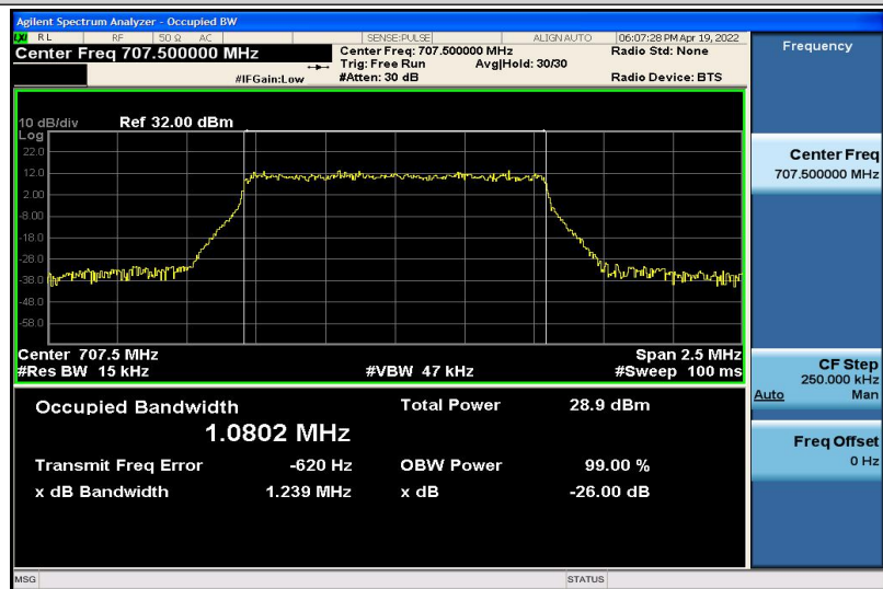
Band12-1.4MHz-16QAM-23095-6RB#0-1.0802
