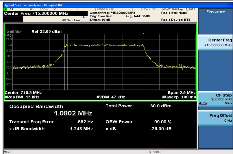
Band12-1.4MHz-QPSK-23173-6RB#0-1.0802
