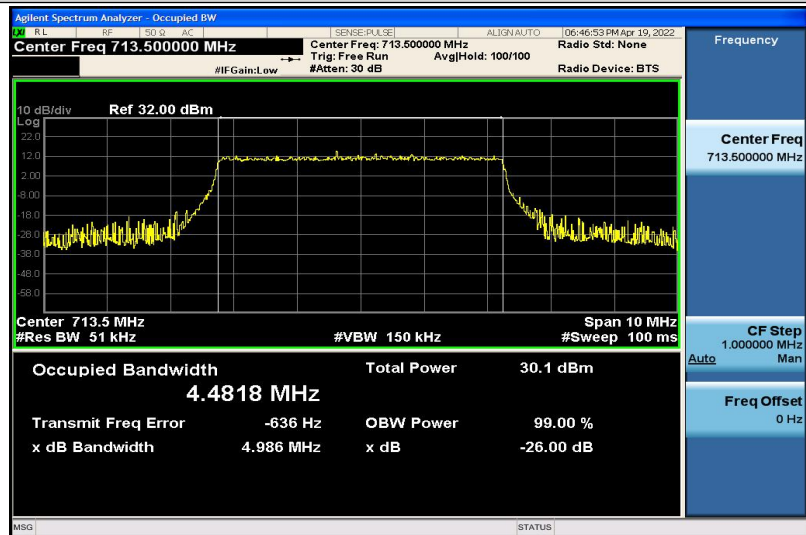
Band12-5MHz-16QAM-23155-25RB#0-4.4818
