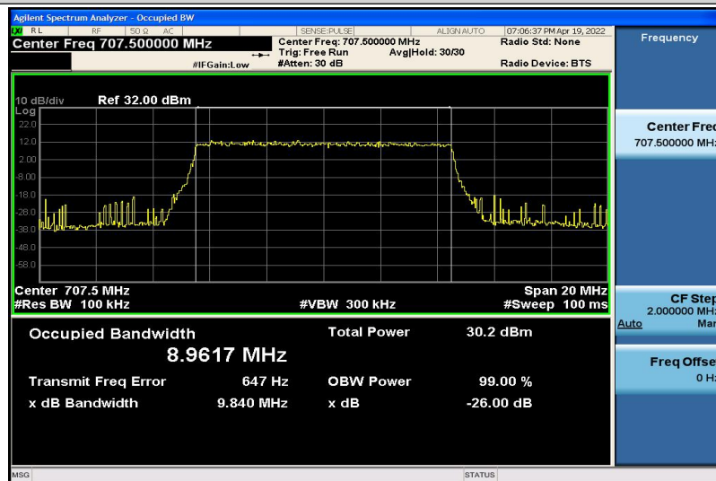
Band12-10MHz-16QAM-23095-50RB#0-8.9617
