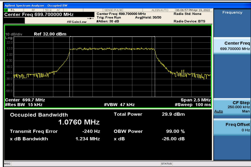
Band12-1.4MHz-QPSK-23017-6RB#0-1.0760
