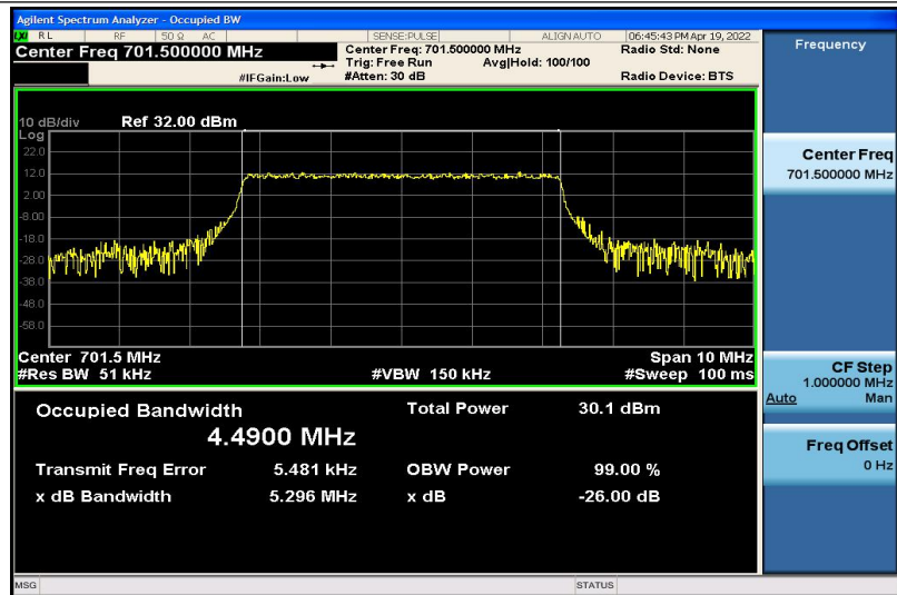
Band12-5MHz-16QAM-23035-25RB#0-4.4900
