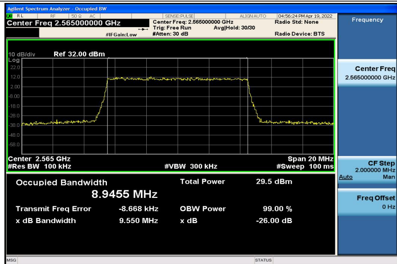
Band7-10MHz-16QAM-21400-50RB#0-8.9455
