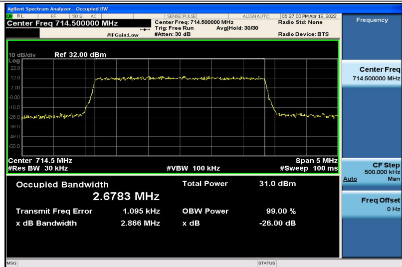
Band12-3MHz-QPSK-23165-15RB#0-2.6783
