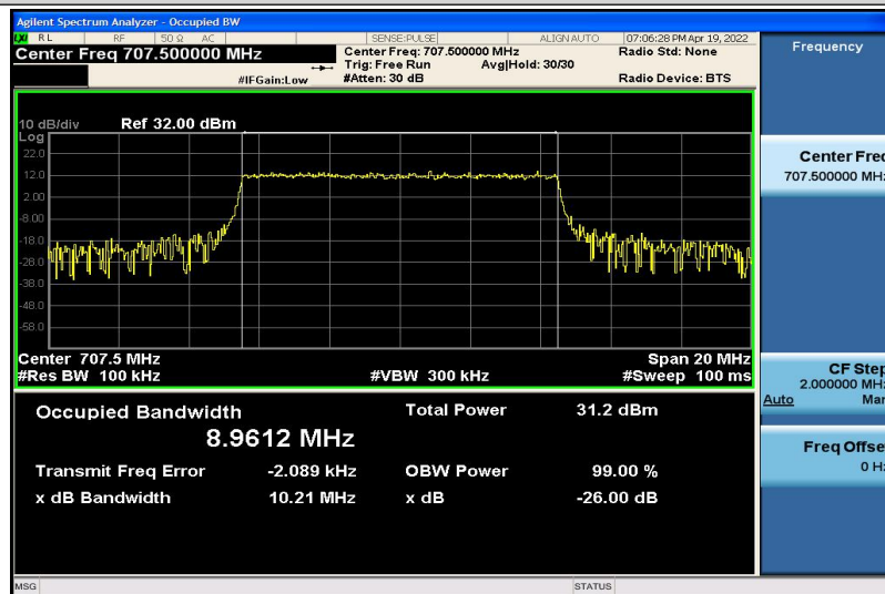
Band12-10MHz-QPSK-23095-50RB#0-8.9612
