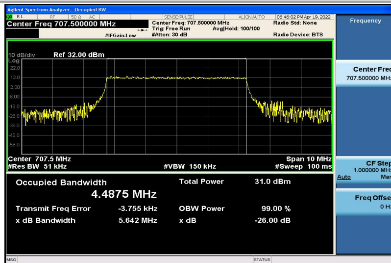
Band12-5MHz-QPSK-23095-25RB#0-4.4875
