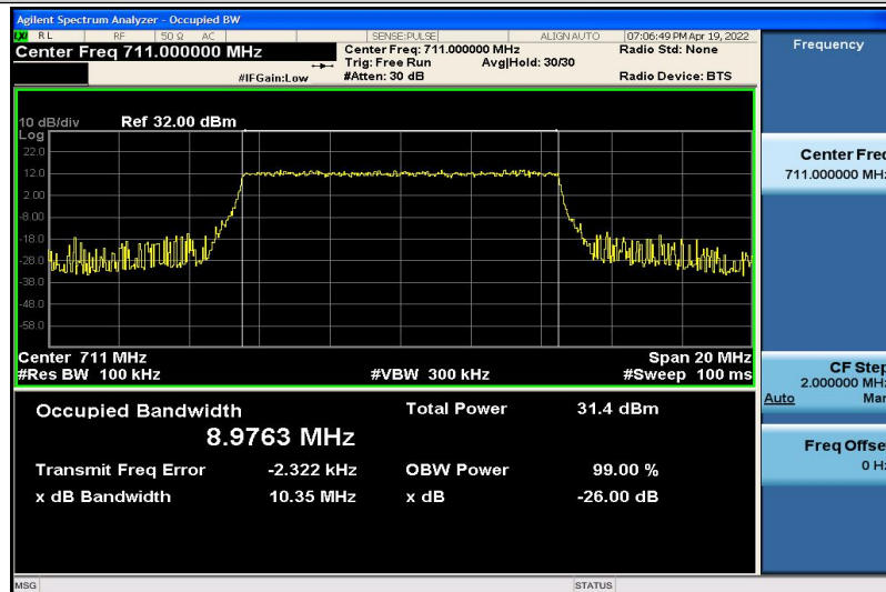
Band12-10MHz-QPSK-23130-50RB#0-8.9763
