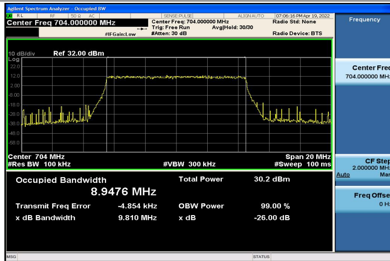
Band12-10MHz-16QAM-23060-50RB#0-8.9476
