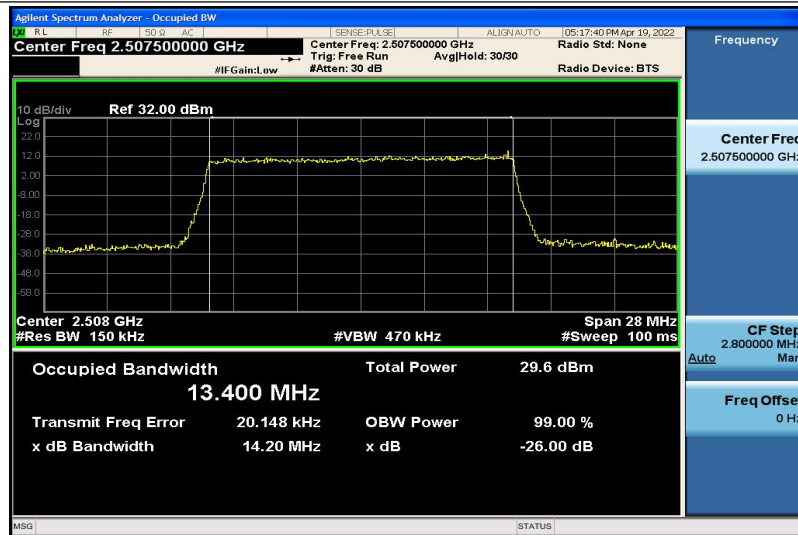
Band7-15MHz-16QAM-20825-75RB#0-13.400
