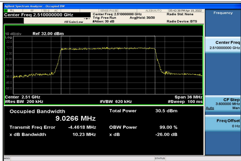
Band7-20MHz-QPSK-20850-100RB#0-9.0266
