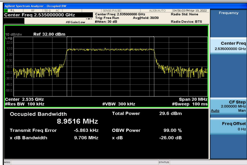
Band7-10MHz-16QAM-21100-50RB#0-8.9516
