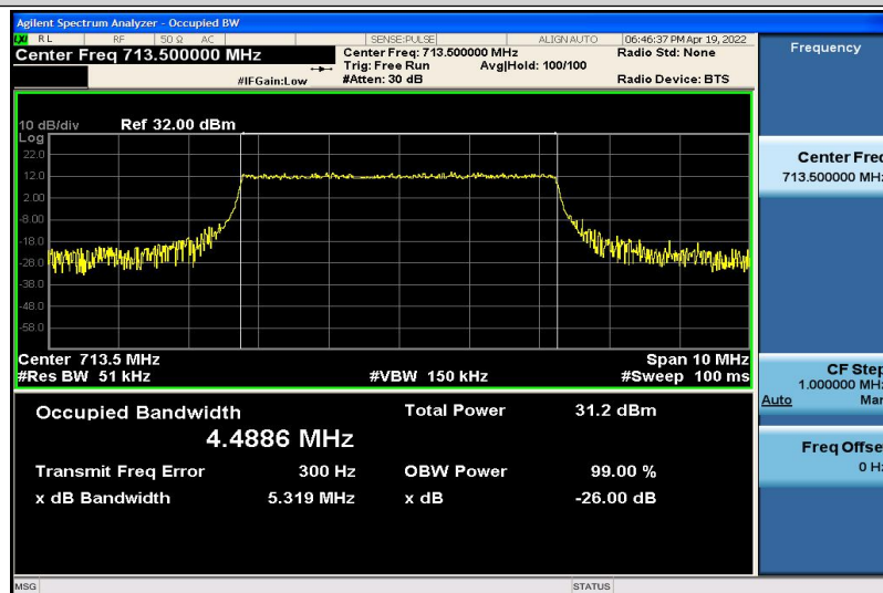
Band12-5MHz-QPSK-23155-25RB#0-4.4886
