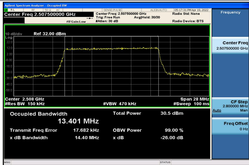
Band7-15MHz-QPSK-20825-75RB#0-13.401
