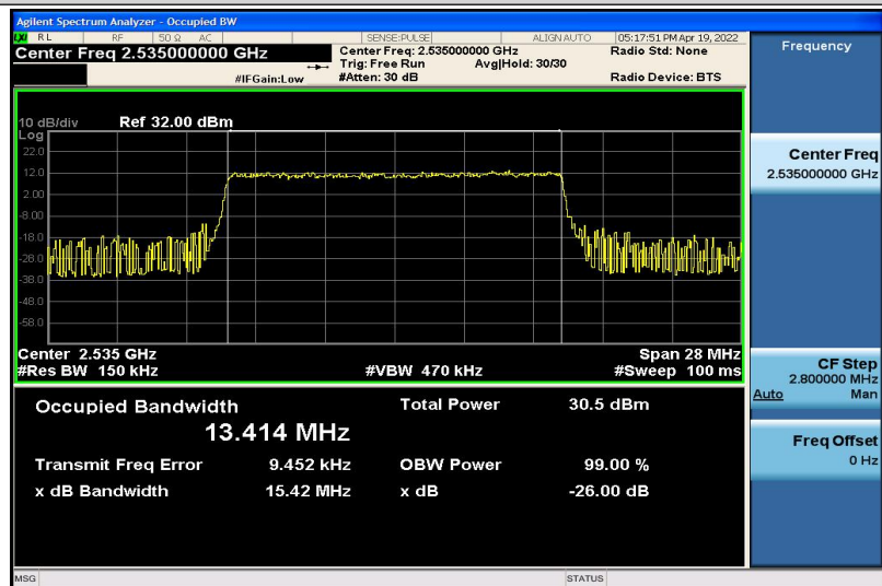
Band7-15MHz-QPSK-21100-75RB#0-13.414
