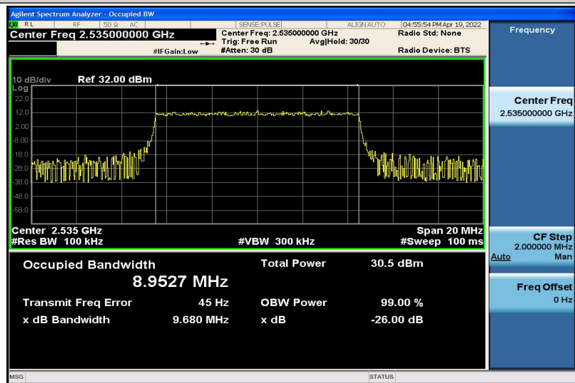
Band7-10MHz-QPSK-21100-50RB#0-8.9527
