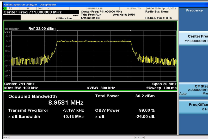
Band12-10MHz-16QAM-23130-50RB#0-8.9581
