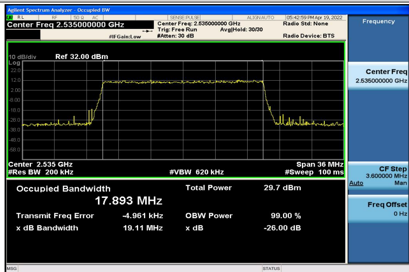
Band7-20MHz-QPSK-21100-100RB#0-17.893
