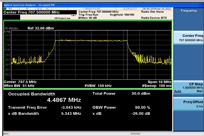
Band12-5MHz-16QAM-23095-25RB#0-4.4867
