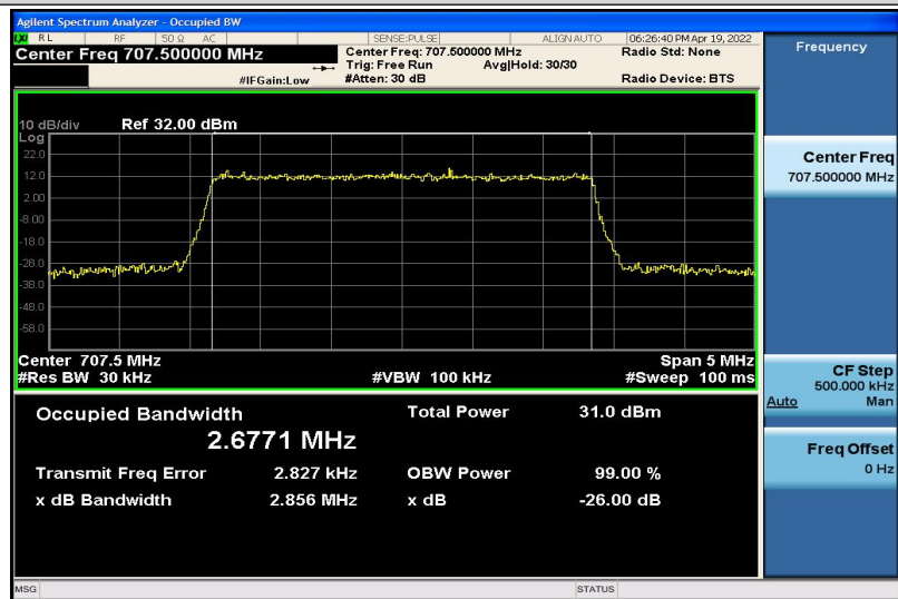
Band12-3MHz-QPSK-23095-15RB#0-2.6771
