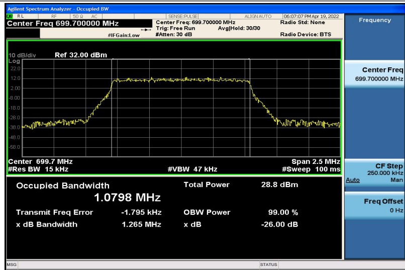
Band12-1.4MHz-16QAM-23017-6RB#0-1.0798
