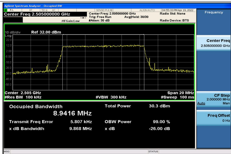
Band7-10MHz-QPSK-20800-50RB#0-8.9416
