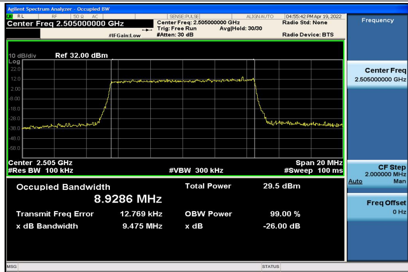
Band7-10MHz-16QAM-20800-50RB#0-8.9286
