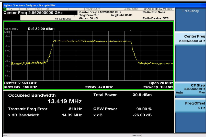
Band7-15MHz-QPSK-21375-75RB#0-13.419
