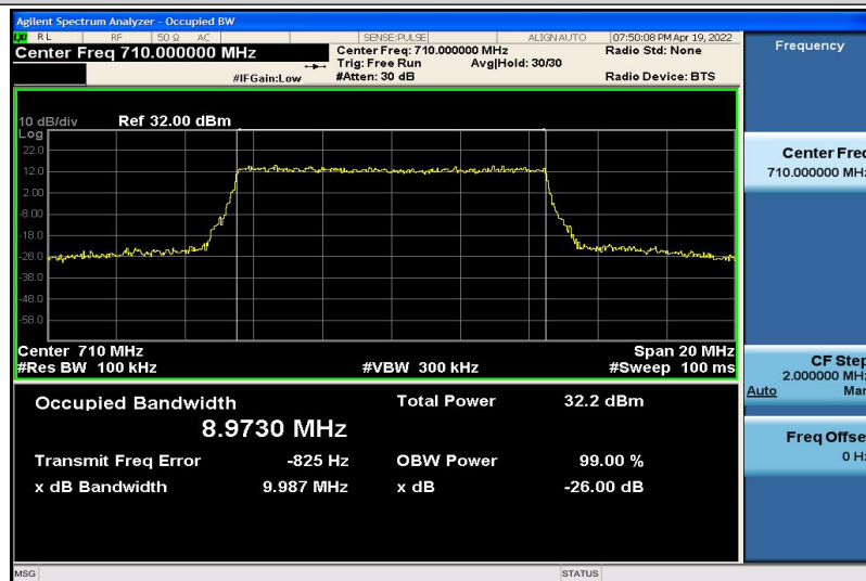
Band17-10MHz-QPSK-23790-50RB#0-8.9730
