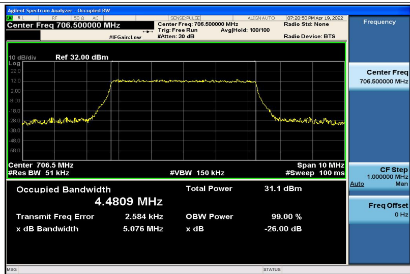
Band17-5MHz-16QAM-23755-25RB#0-4.4809
