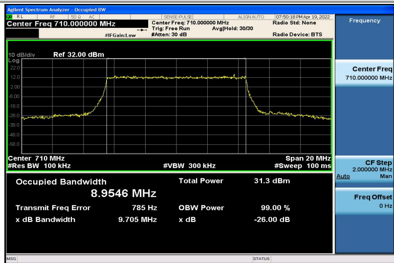
Band17-10MHz-16QAM-23790-50RB#0-8.9546
