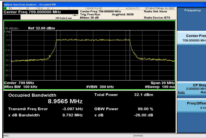
Band17-10MHz-QPSK-23780-50RB#0-8.9565
