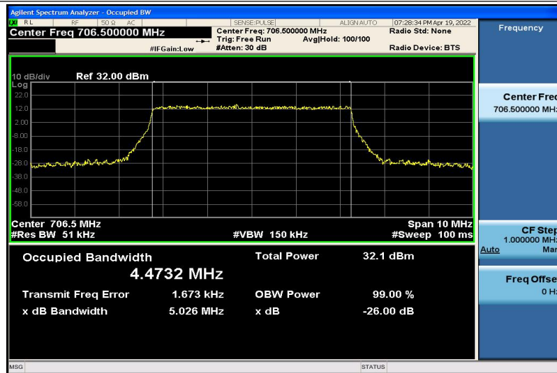
Band17-5MHz-QPSK-23755-25RB#0-4.4732
