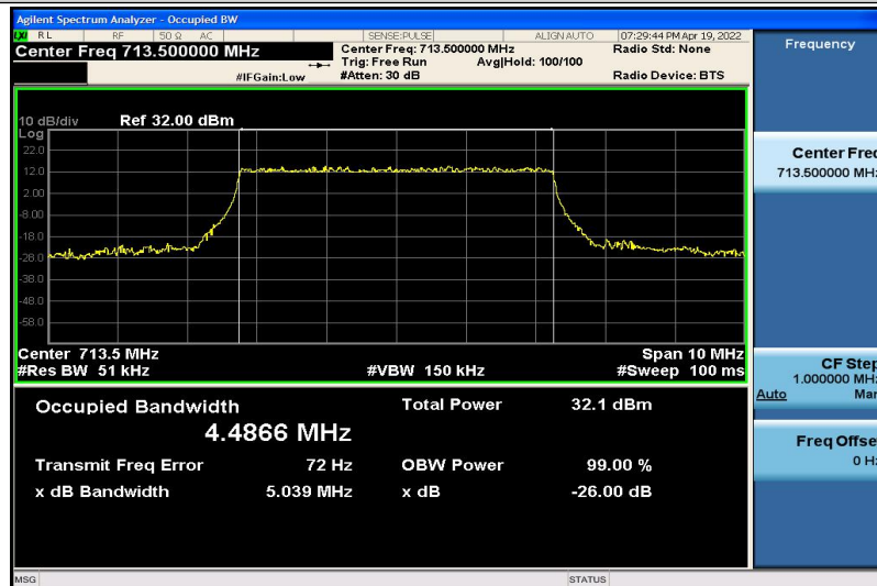
Band17-5MHz-QPSK-23825-25RB#0-4.4866
