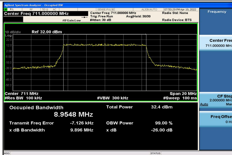
Band17-10MHz-QPSK-23800-50RB#0-8.9548
