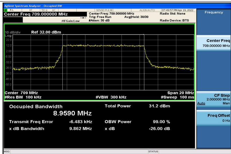
Band17-10MHz-16QAM-23780-50RB#0-8.9590
