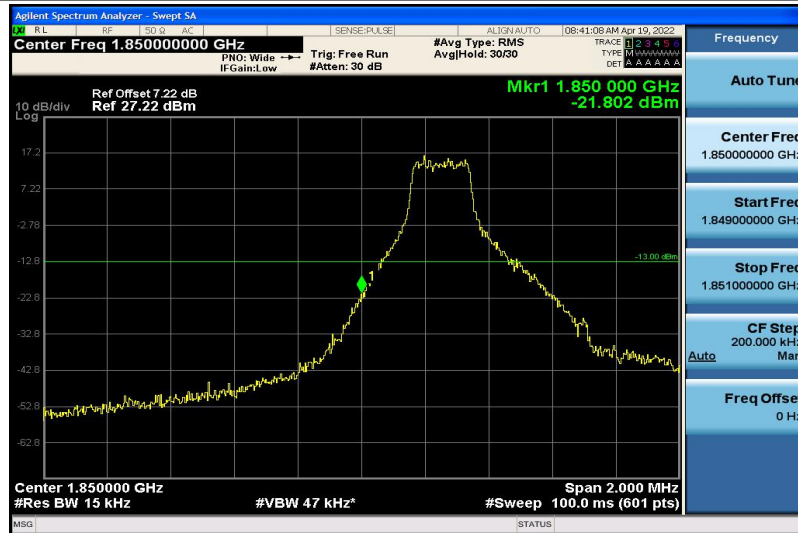
Band2-1.4MHz-QPSK-18607-1RB#0
