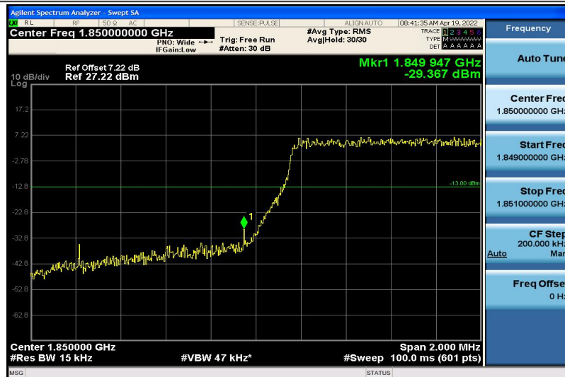
Band2-1.4MHz-16QAM-18607-6RB#0
