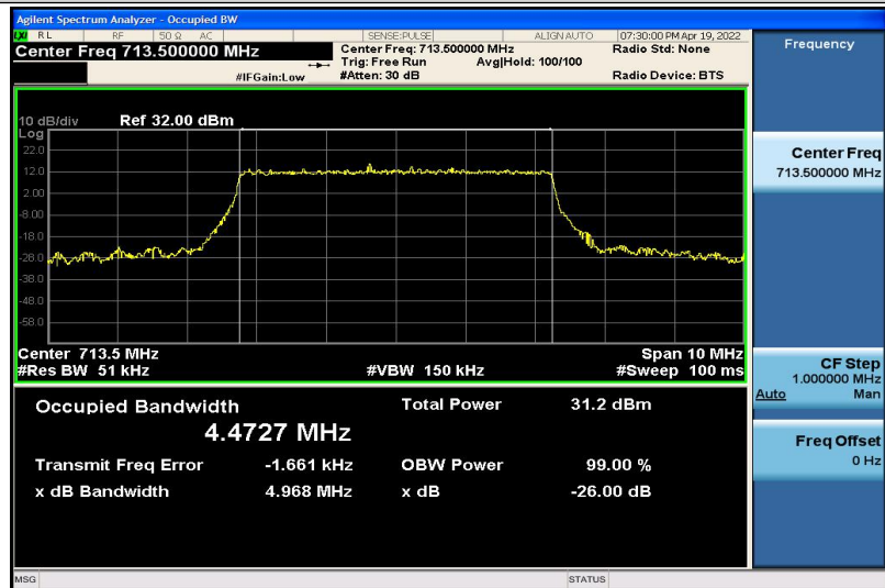
Band17-5MHz-16QAM-23825-25RB#0-4.4727
