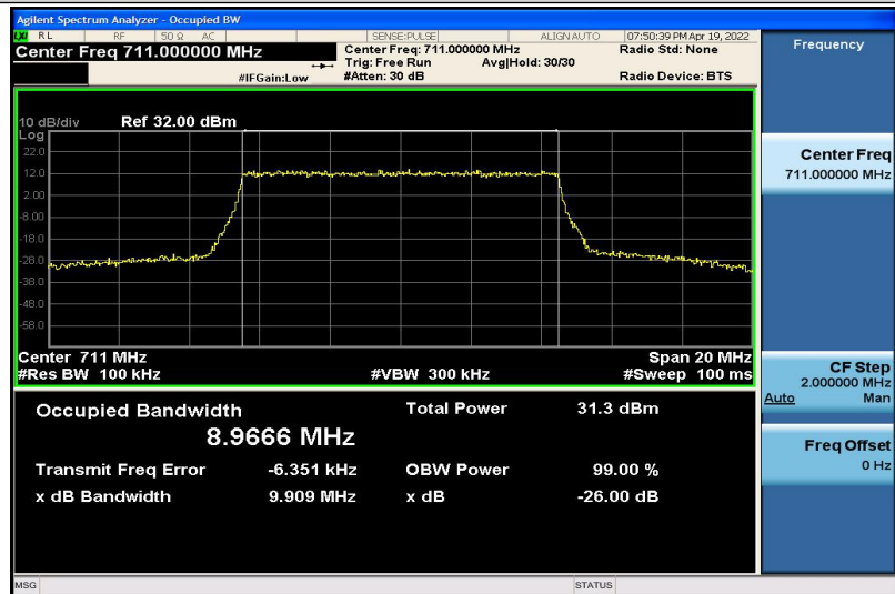
Band17-10MHz-16QAM-23800-50RB#0-8.9666
