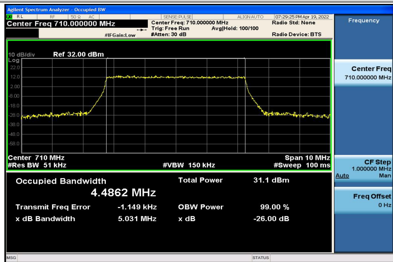
Band17-5MHz-16QAM-23790-25RB#0-4.4862
