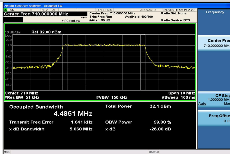
Band17-5MHz-QPSK-23790-25RB#0-4.4851
