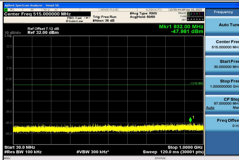
Band2-3MHz-16QAM-19185-1RB#0-30~1000MHz
