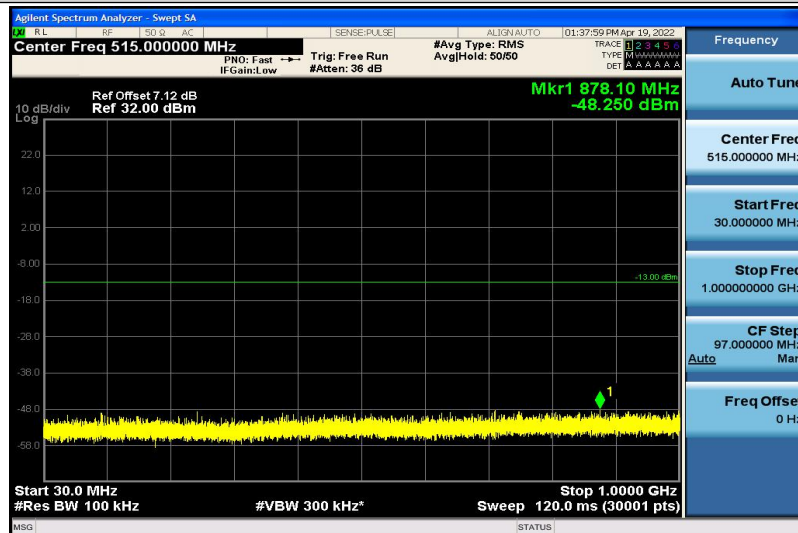
Band4-5MHz-16QAM-20375-1RB#0-30~1000MHz
