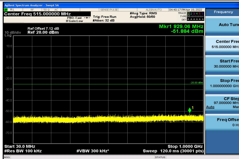
Band7-5MHz-16QAM-21425-1RB#0-30~1000MHz
