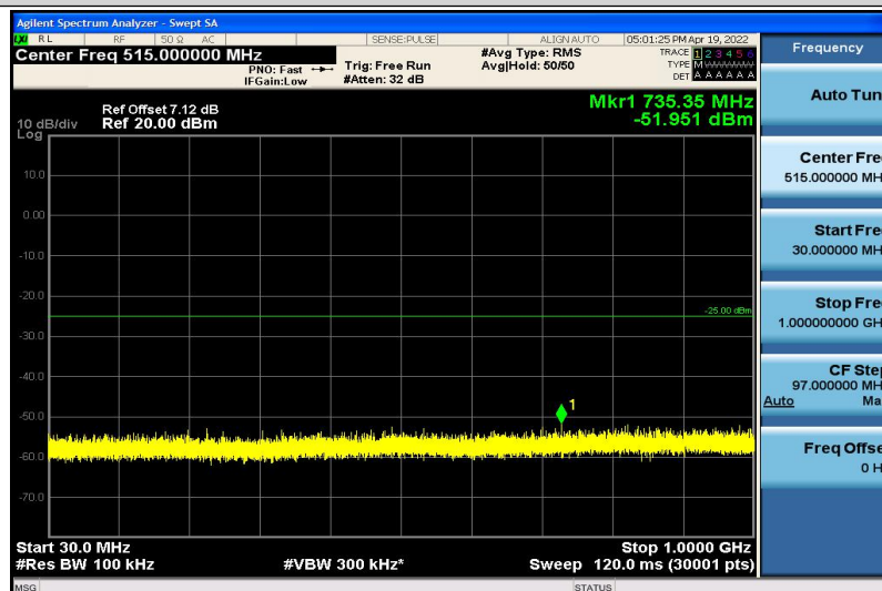
Band7-10MHz-16QAM-21400-1RB#0-30~1000MHz
