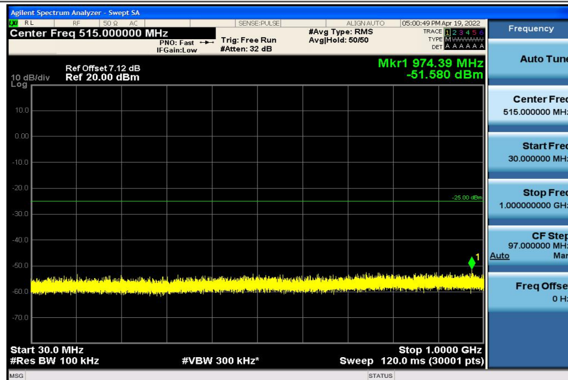
Band7-10MHz-QPSK-21400-1RB#0-30~1000MHz
