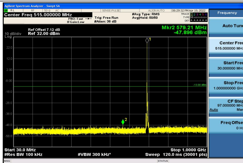
Band12-3MHz-16QAM-23025-1RB#0-30~1000MHz
