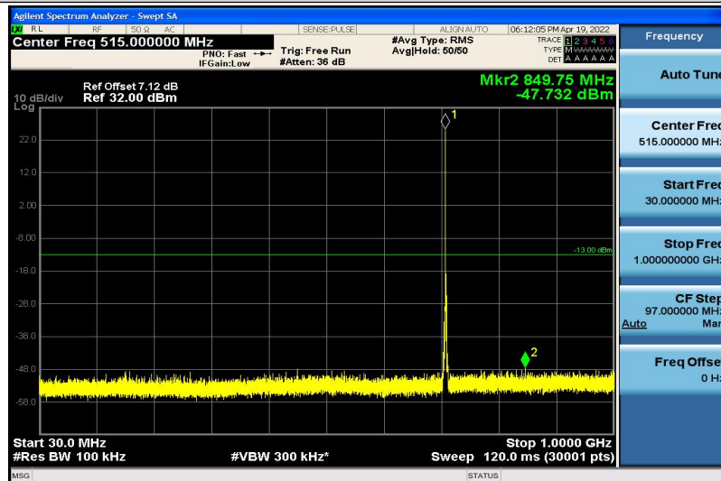
Band12-1.4MHz-QPSK-23173-1RB#0-30~1000MHz
