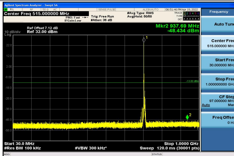
Band12-5MHz-16QAM-23155-1RB#0-30~1000MHz
