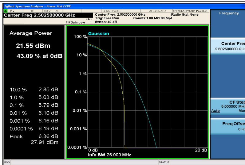
Band7-5MHz-16QAM-20775-1RB#0
