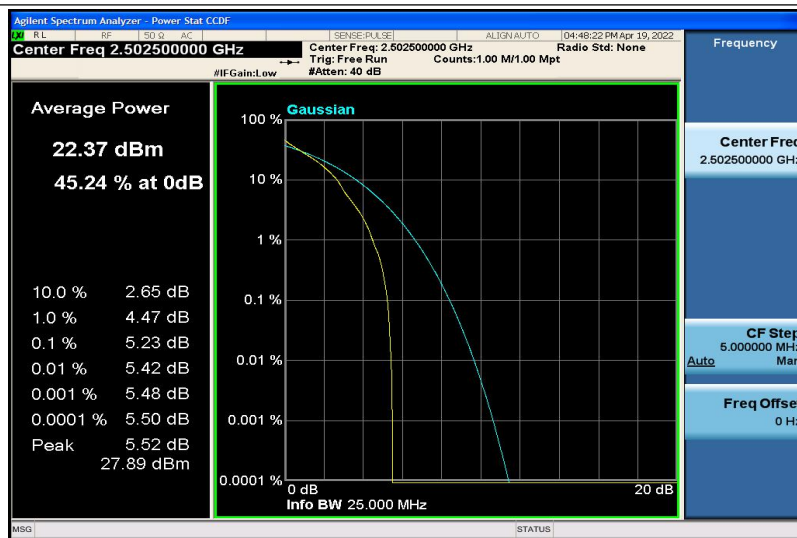
Band7-5MHz-QPSK-20775-1RB#0
