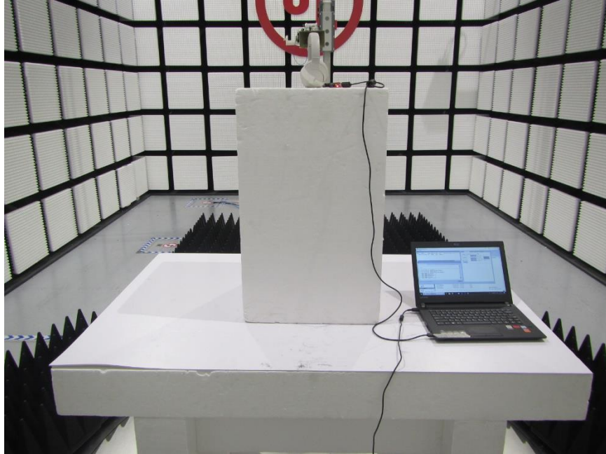
MEASUREMENT POSITION
