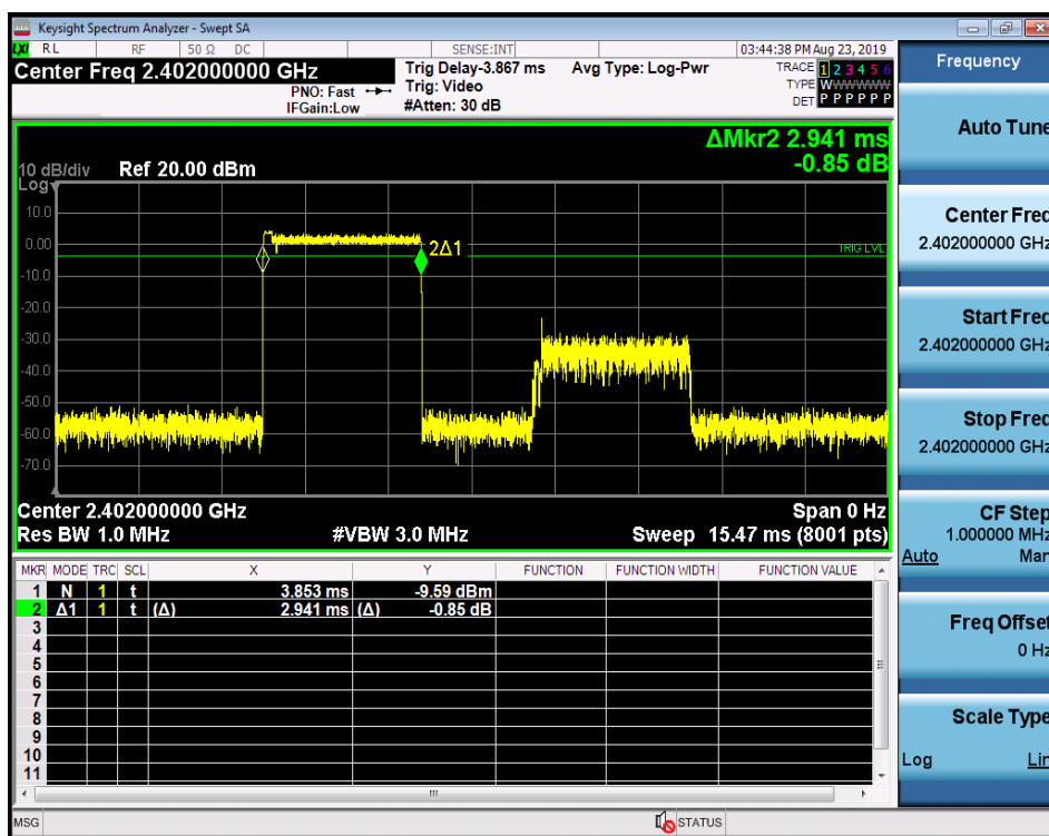
Dwell Time_3DH5_2402
