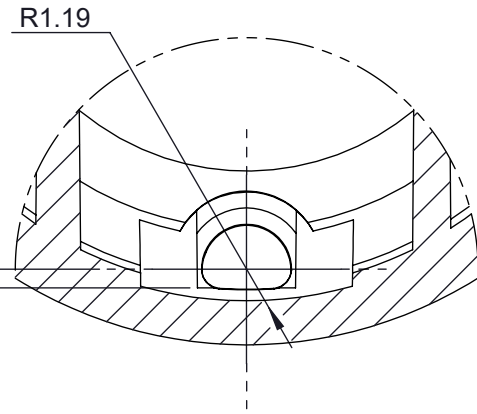
DETAIL F SCALE 5 : 1
