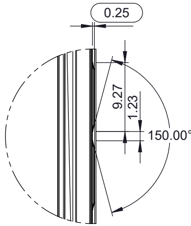
DETAIL R SCALE 2 : 1
