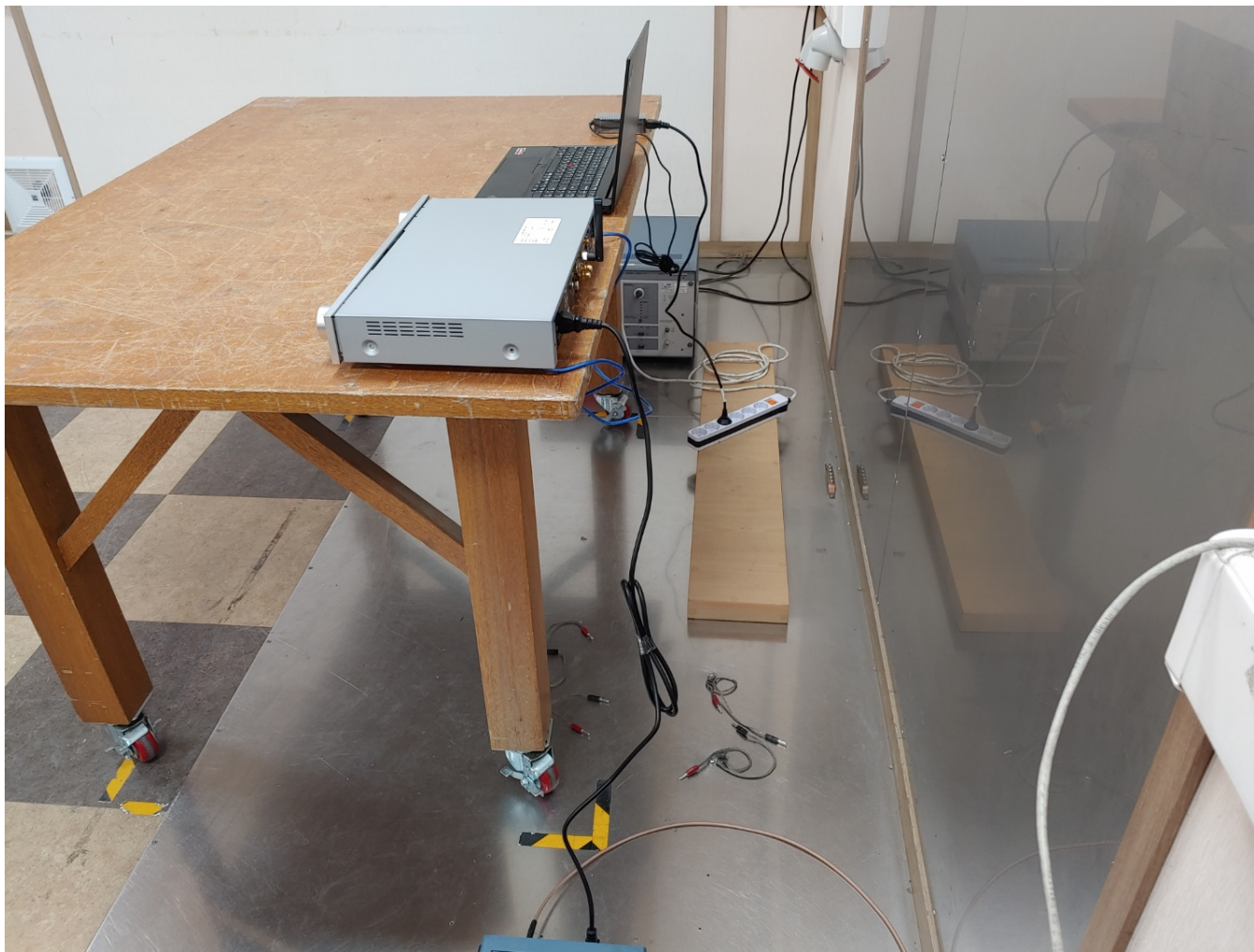
AC Conducted measurement (Rear view)
