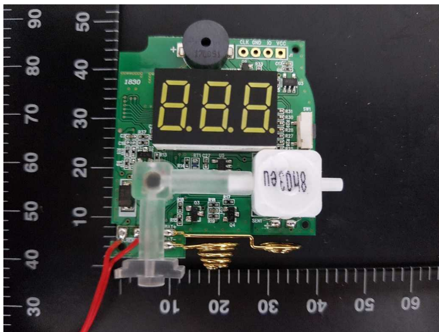
Main board - Rear Bottom
