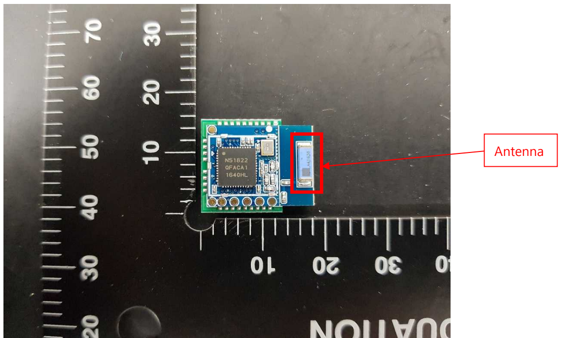
Bluetooth Module - Front Top (Remove the shielding cover)
