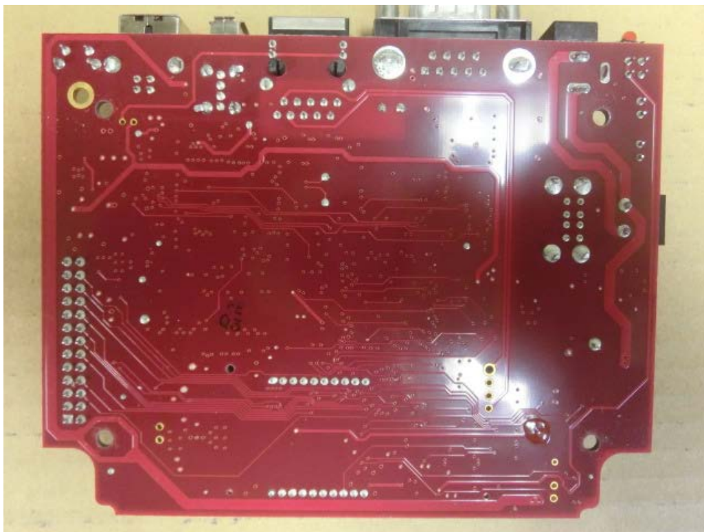
TS-7533(Soldering Side)
