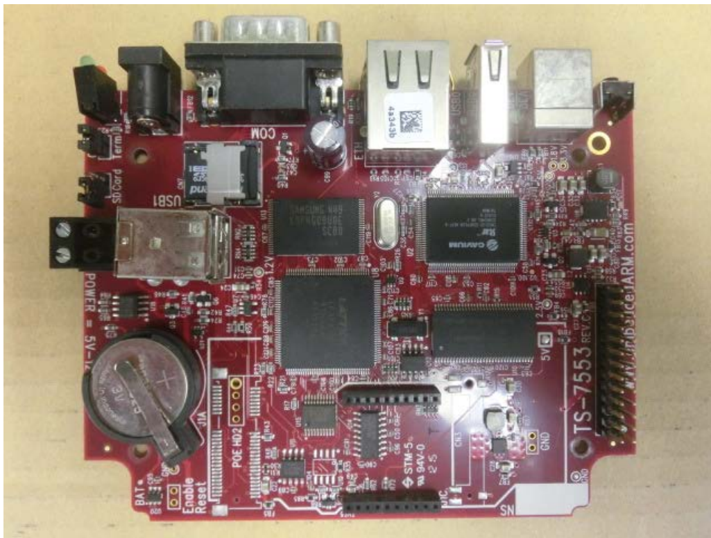
TS-7533(Component Side)
