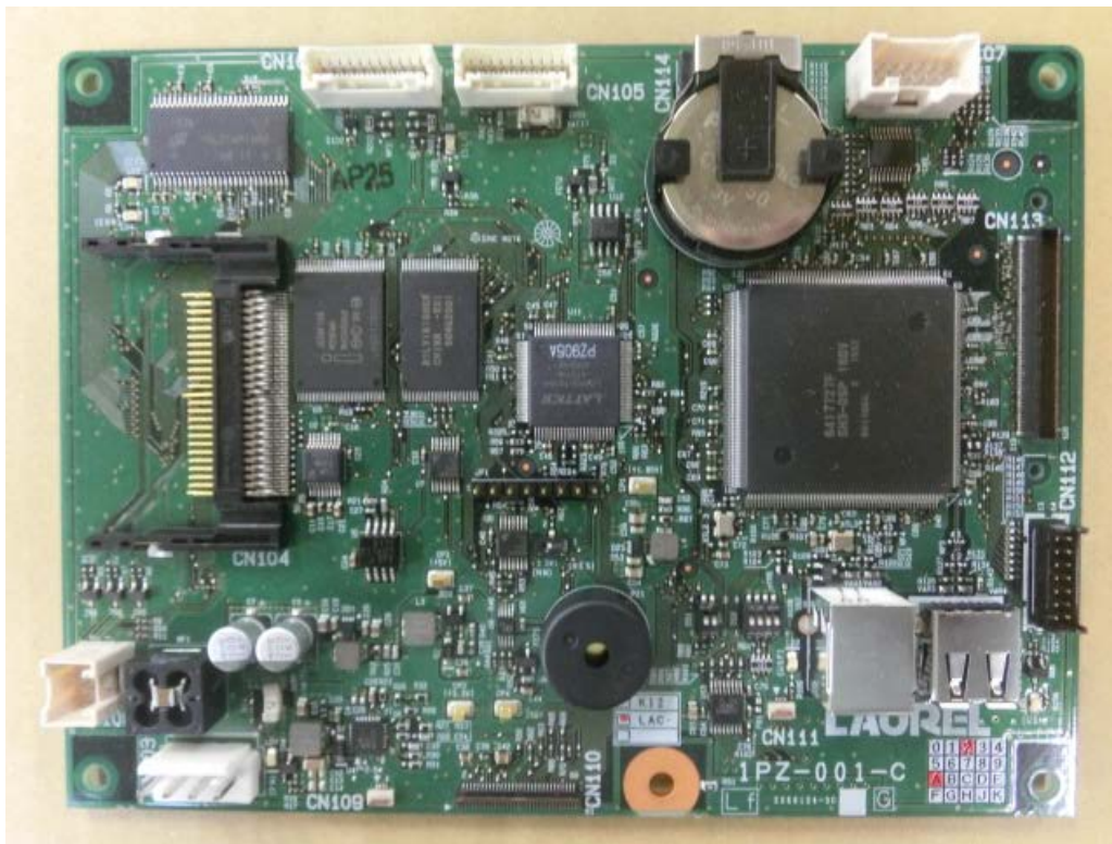
1PZ-001-C (Component Side)
