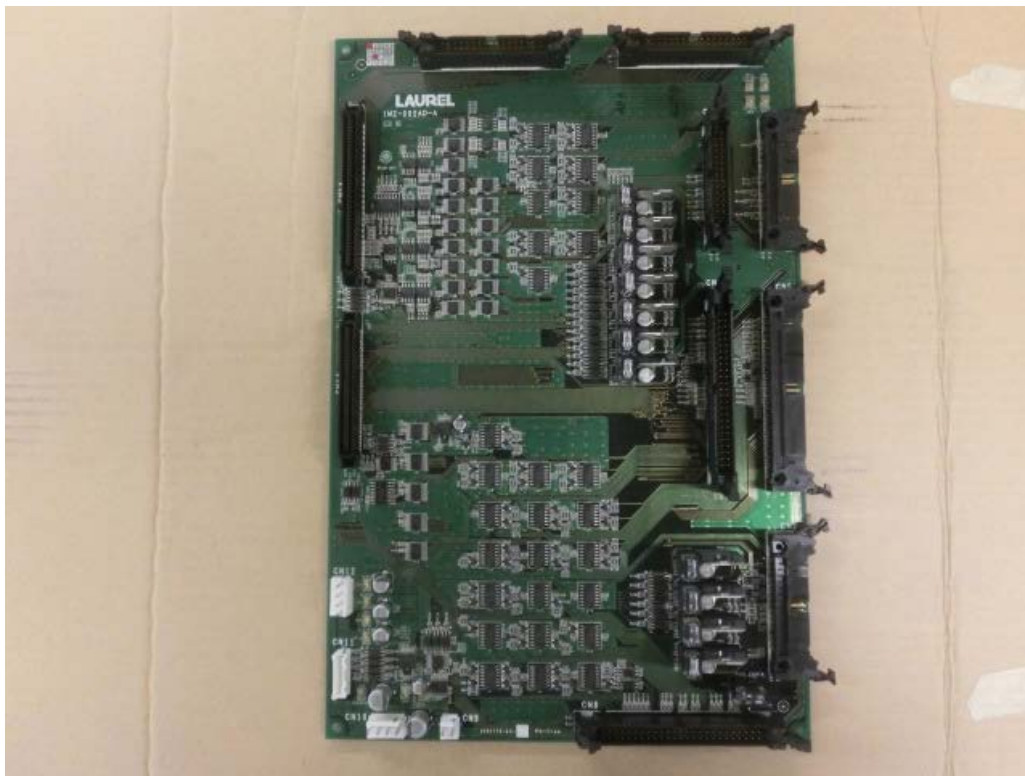
1MZ-002AD-A (Component Side)
