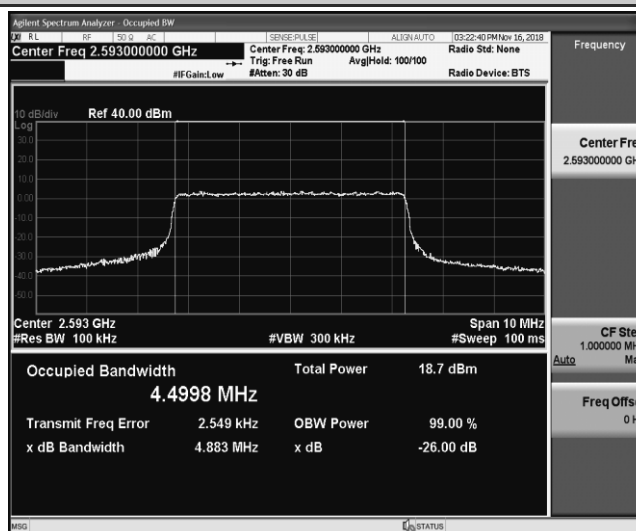
Band41_5MHz_QPSK_41315_25RB#0
