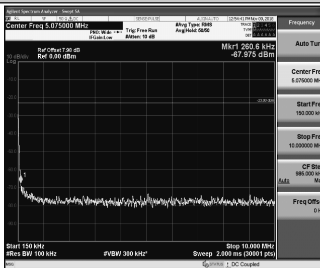
Band5_5MHz_QPSK_20625_1RB#0
