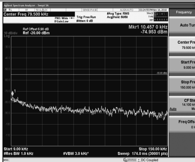
Band41_5MHz_QPSK_40265_1RB#0
