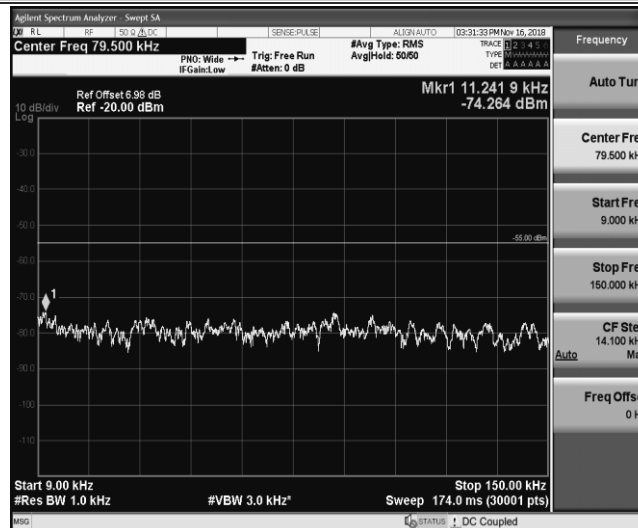
Band41_5MHz_QPSK_41315_1RB#0
