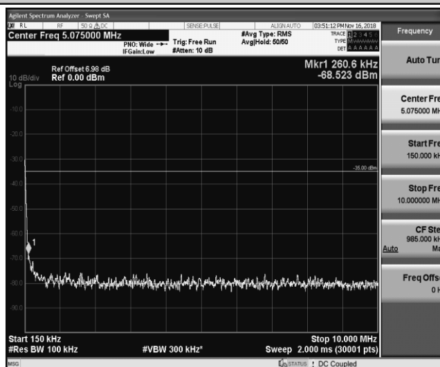
Band41_10MHz_16QAM_40290_1RB#0
