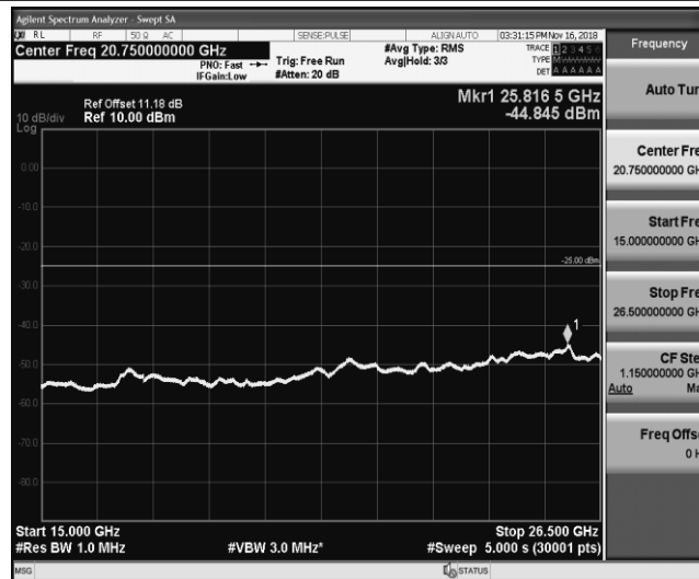
Band41_5MHz_16QAM_41315_1RB#0
