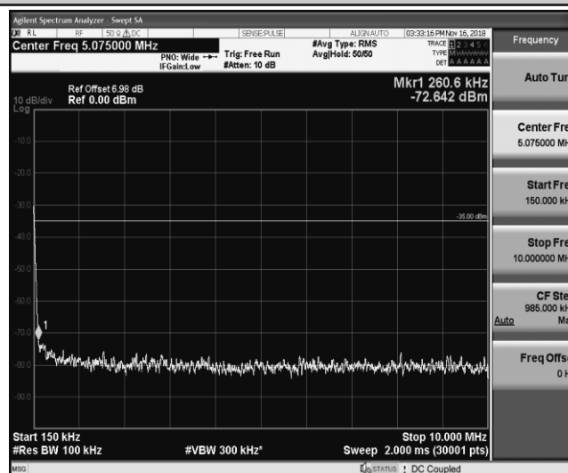
Band41_5MHz_16QAM_41315_1RB#0
