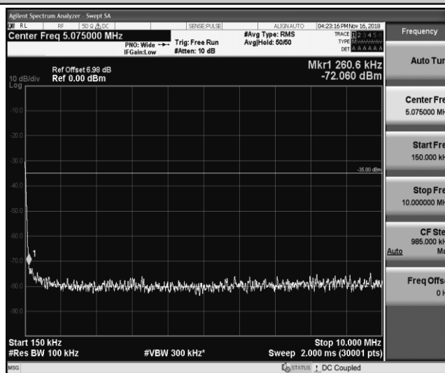
Band41_15MHz_QPSK_41165_1RB#0
