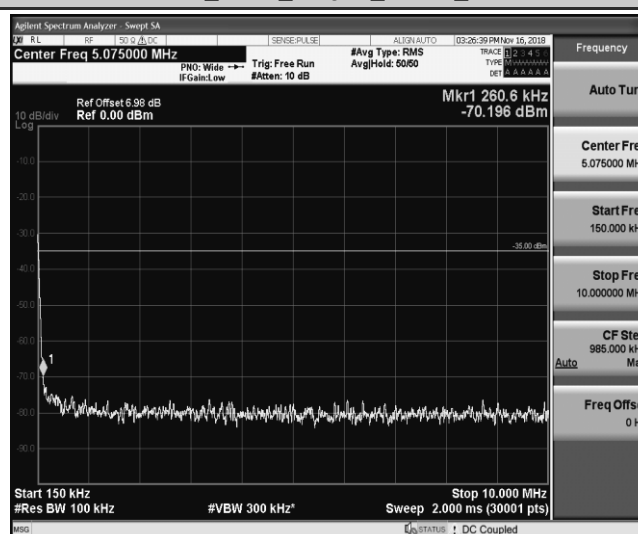
Band41_5MHz_16QAM_40265_1RB#0
