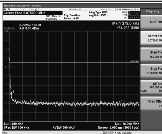
Band41_5MHz_QPSK_41315_1RB#0
