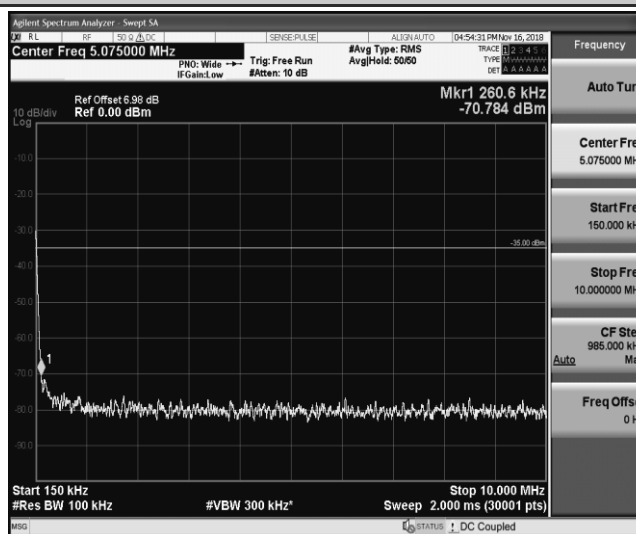
Band41_20MHz_16QAM_41140_1RB#0
