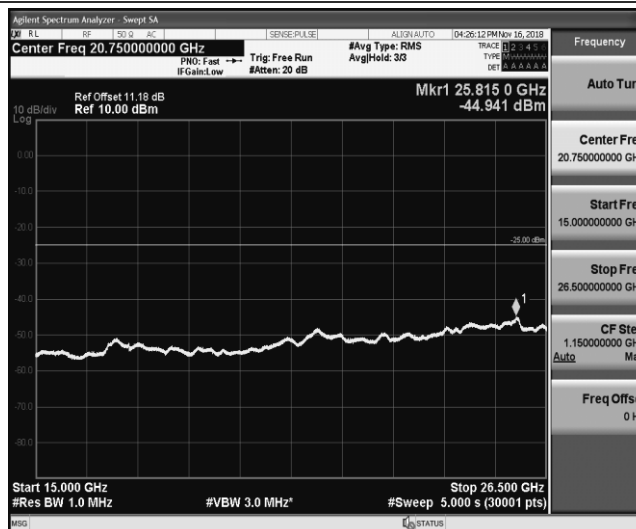
Band41_20MHz_QPSK_40340_1RB#0
