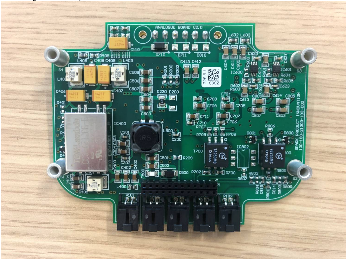
C – Analogue Board - Top
