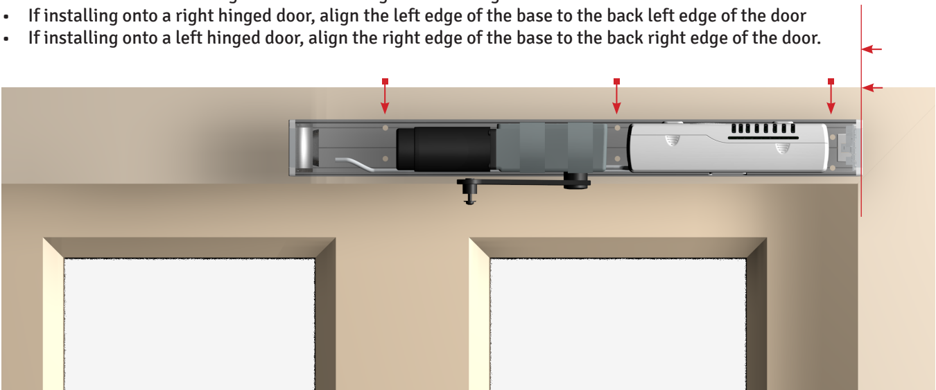
AutoSwing with Push Arm on left hinged door (back view, hinges are on the right)
