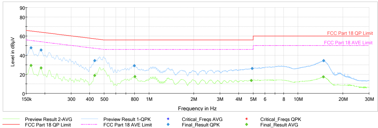
Plot 6-5. AC Line-Conducted Plot with WPT (N, with AC/DC adapter)
