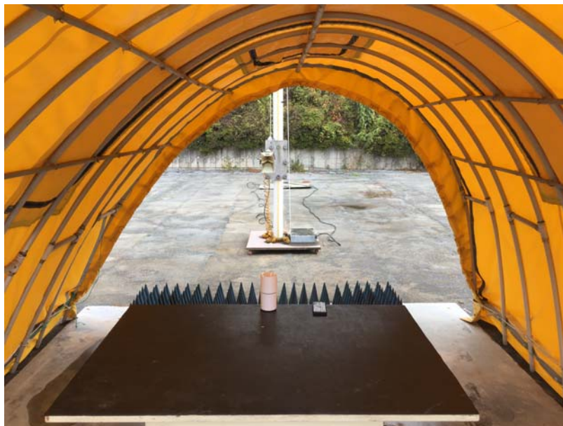
Photograph 2 : Setup for radiated Emissions (above 1 GHz)
