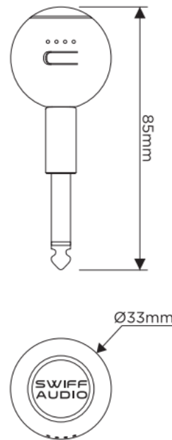
Product Dimensions
