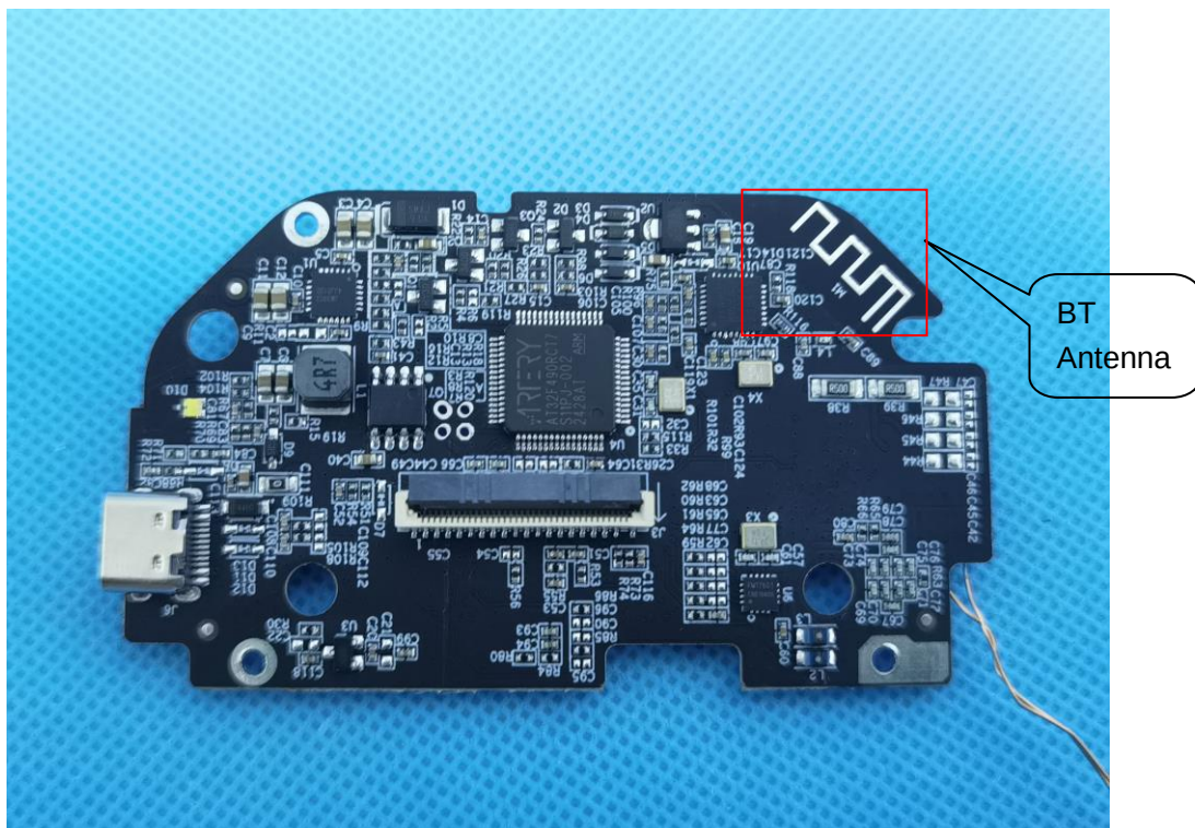
Internal view-6 of EUT
