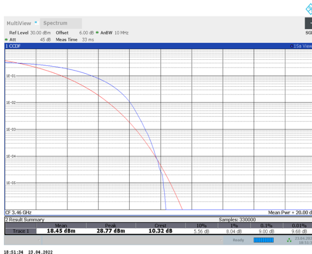
Band42-20MHz-QPSK-42590-100RB#0
