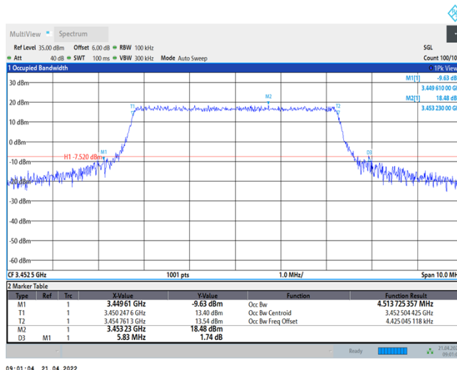
Band42-5MHz-QPSK-42590-25RB#0
