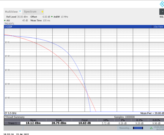
Band42-20MHz-QPSK-42590-100RB#0
