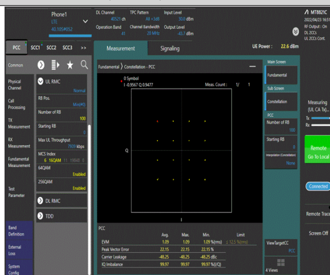
41-41-20MHz-20MHz-16QAM-16QAM-40521-40719-100RB#0-100RB#0
