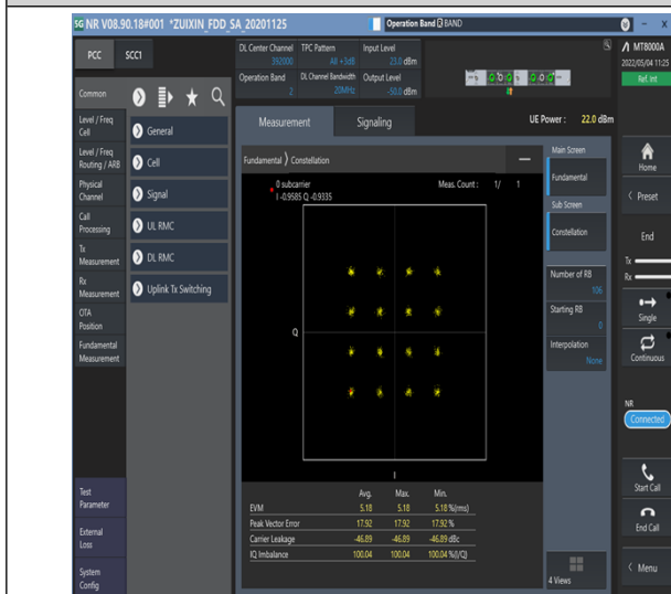
1-N2-PC3-15-20-M-7-CP-16QAM-Outer_Full-106@0-Ant1-see graph-PASS
