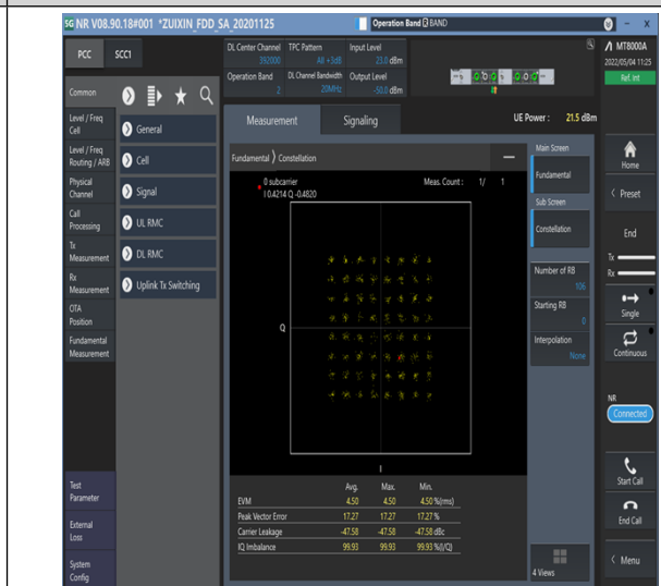
1-N2-PC3-15-20-M-8-CP-64QAM-Outer_Full-106@0-Ant1-see graph-PASS
