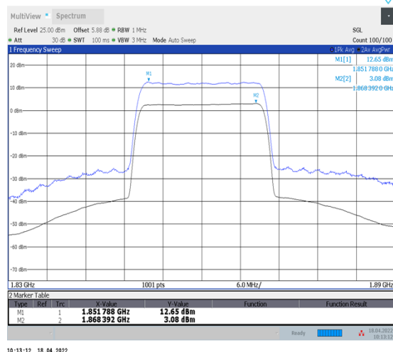
1-N2--15-20-L-2-CP-256QAM-Outer_Full-106@0- Ant1-9.57-100%-0.00-9.57-PASS≤13
