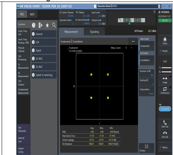
1-N2-PC3-15-20-M-6-CP-QPSK-Outer_Full-106@0-Ant1-see graph-PASS
