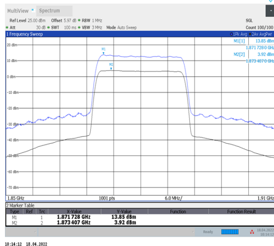
1-N2--15-20-M-2-CP-256QAM-Outer_Full-106@0- Ant1-9.93-100%-0.00-9.93-PASS≤13
