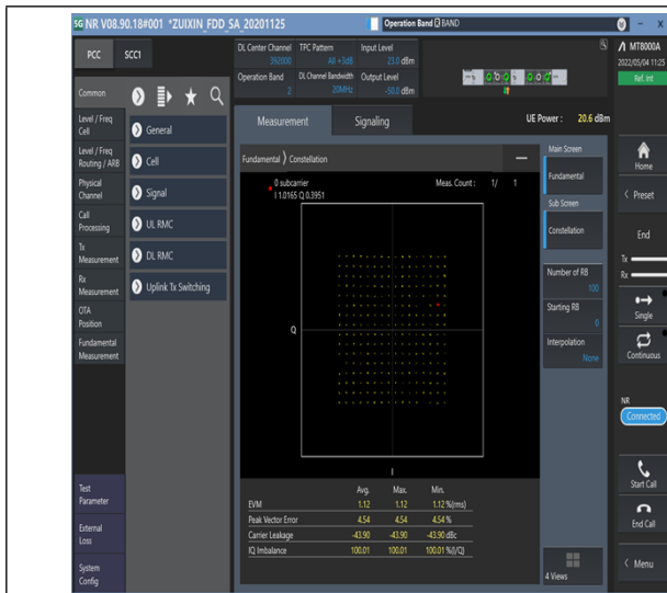
1-N2-PC3-15-20-M-5-DFT-256QAM-Outer_Full-100@0-Ant1-see graph-PASS
