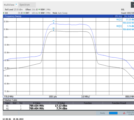
1-N14--15-10-M-2-CP-256QAM-Outer_Full-52@0- Ant1-9.39-100%-0.00-9.39-PASS-≤13
