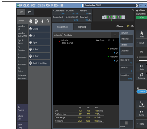
1-N14-PC3-15-10-M-1-DFT-PI2BPSK-Outter_Full-50@0-Ant1-see graph-PASS
