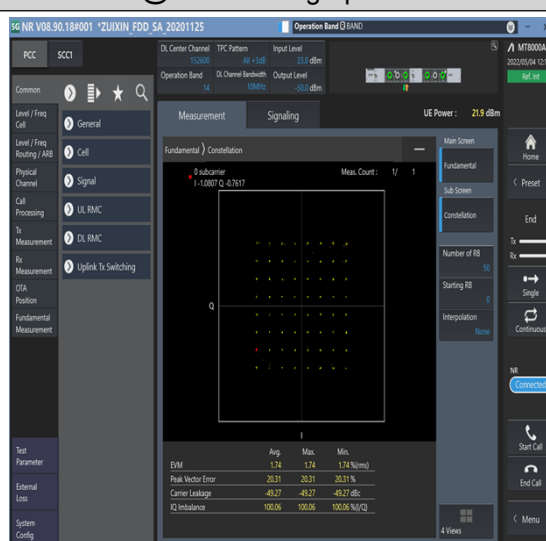
1-N14-PC3-15-10-M-4-DFT-64QAM-Outter_Full-50@0-Ant1-see graph-PASS
