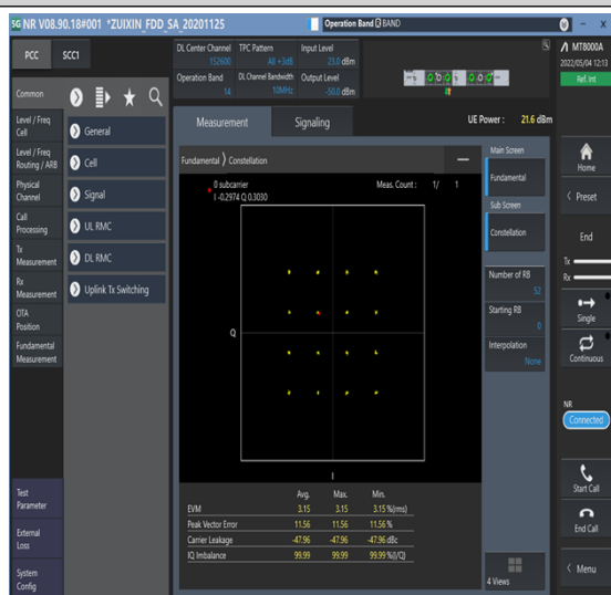
1-N14-PC3-15-10-M-7-CP-16QAM-Outer_Full-52@0-Ant1-see graph-PASS
