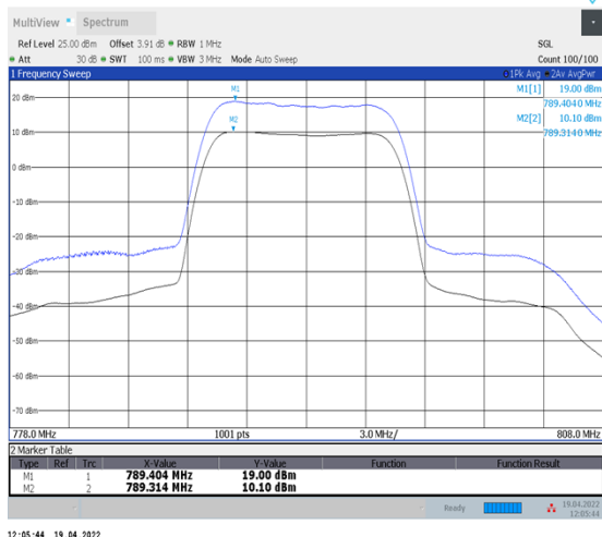
1-N14--15-10-L-1-DFT-256QAM-Outer_Full-50@0- Ant1-8.90-100%-0.00-8.90-PASS-≤13
