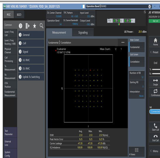
1-N14-PC3-15-10-M-8-CP-64QAM-Outer_Full-52@0-Ant1-see graph-PASS
