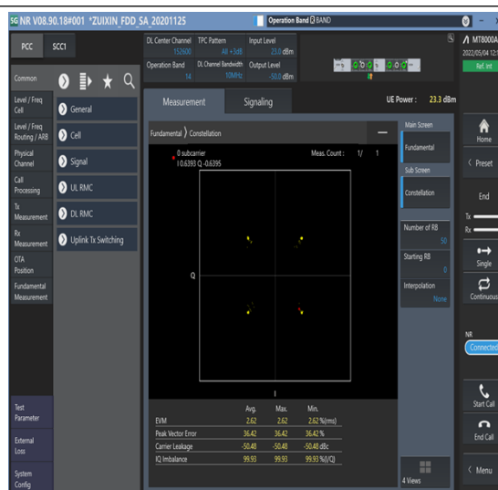
1-N14-PC3-15-10-M-2-DFT-QPSK-Outter_Full-50@0-Ant1-see graph-PASS
