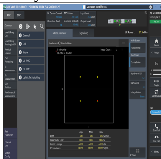
1-N14-PC3-15-10-M-6-CP-QPSK-Outer_Full-52@0-Ant1-see graph-PASS
