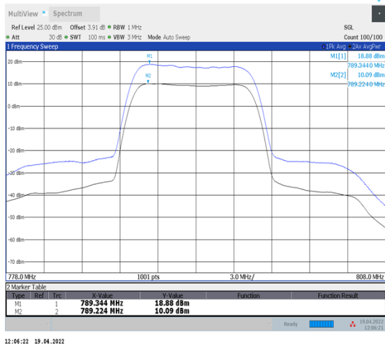
1-N14--15-10-M-1-DFT-256QAM-Outer_Full-50@0- Ant1-8.79-100%-0.00-8.79-PASS-≤13
