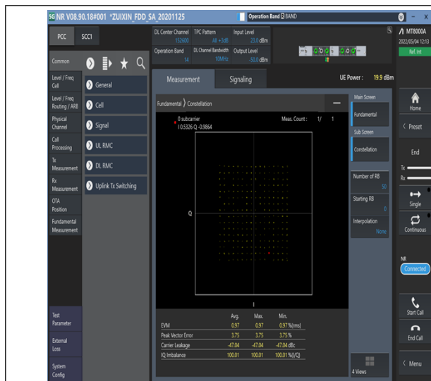
1-N14-PC3-15-10-M-5-DFT-256QAM-Outer_Full-50@0-Ant1-see graph-PASS
