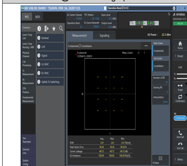
1-N14-PC3-15-10-M-3-DFT-16QAM-Outter_Full-50@0-Ant1-see graph-PASS
