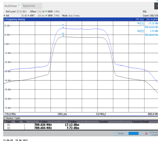
1-N14--15-10-L-2-CP-256QAM-Outer_Full-52@0- Ant1-9.40-100%-0.00-9.40-PASS-≤13
