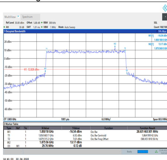
1-N25--15-30-L-7-CP-16QAM-Outet_Full-160@0- Ant1-28.631-29.760-≤30-PASS
