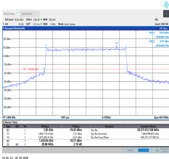
1-N25--15-30-L-8-CP-64QAM-Outet_Full-160@0- Ant1-28.571-29.880-≤30-PASS
