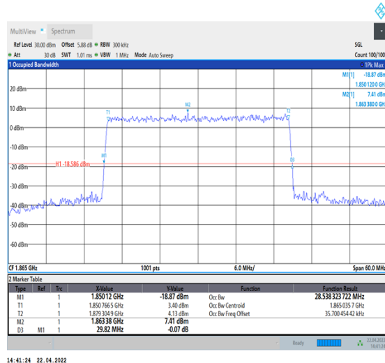
1-N25--15-30-L-9-CP-256QAM-Outet_Full-160@0- Ant1-28.538-29.820-≤30-PASS
