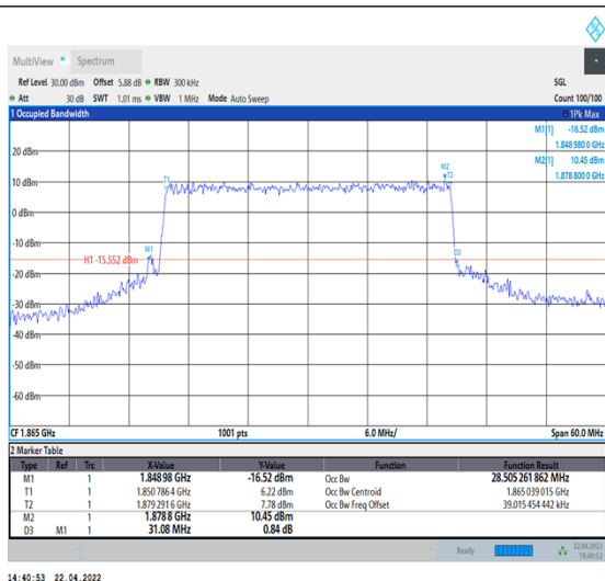
1-N25--15-30-L-6-CP-QPSK-Outet_Full-160@0- Ant1-28.505-31.080-≤30-PASS
