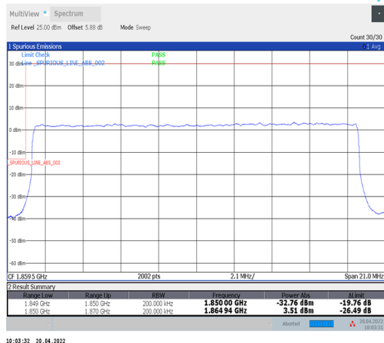
1-N25--15-20-L-3-DFT-PI2BPSK-Outer_Full-100@0-Ant1-seegraph-PASS-see graph
