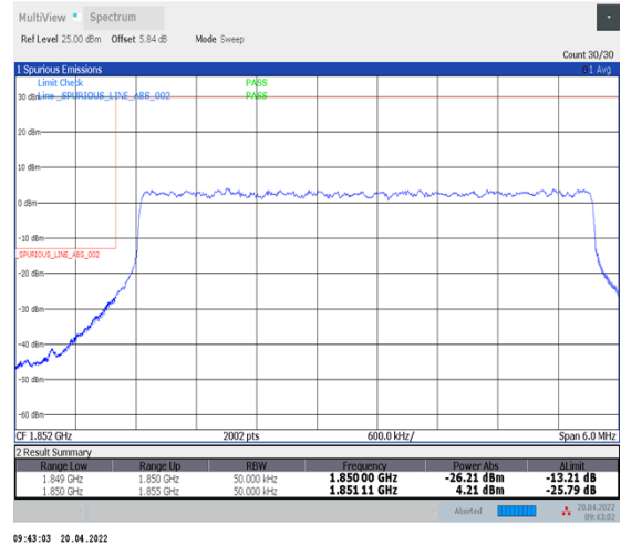
1-N25--15-5-L-3-DFT-PI2BPSK-Outer_Full-25@0-Ant1-seegraph-PASS-see graph
