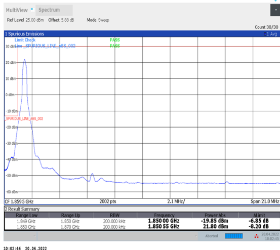
1-N25--15-20-L-1-DFT-PI2BPSK-Edge_1RB_Left-1@0-Ant1-seegraph-PASS-see graph
