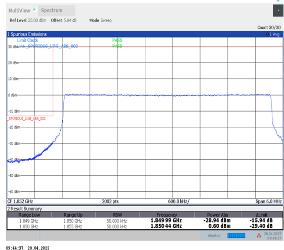
1-N25--15-5-L-6-CP-QPSK-Outer_Full-25@0-Ant1-seegraph-PASS-see graph
