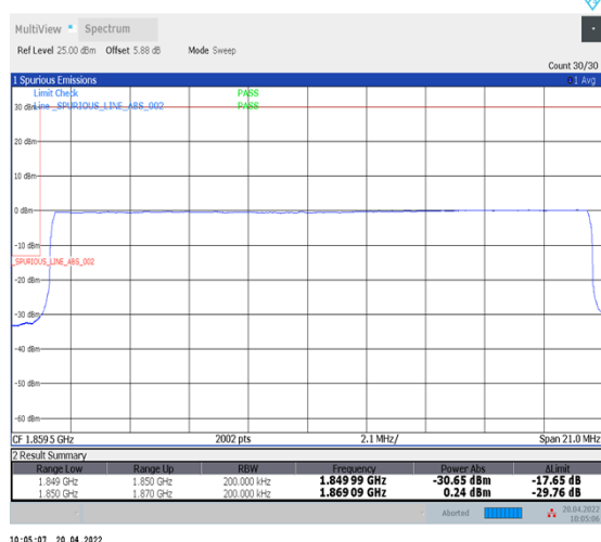
1-N25--15-20-L-6-CP-QPSK-Outer_Full-106@0-Ant1-seegraph-PASS-see graph
