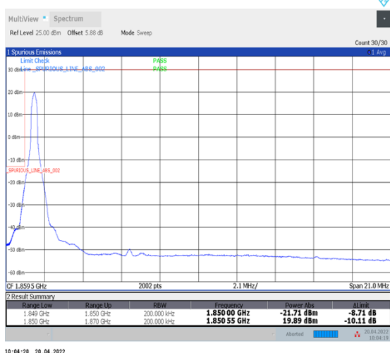
1-N25--15-20-L-4-CP-QPSK-Edge_1RB_Left-1@0-Ant1-seegraph-PASS-see graph
