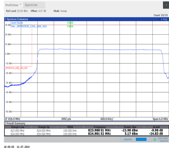
1-N26-824-849--15-5-L-6-CP-QPSK-Outer_Full-25@0-Ant1-seegraph-PASS-see graph
