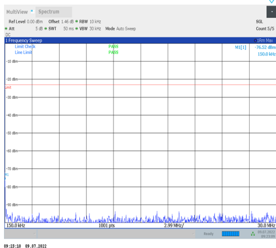
1-N26-824-849-PC3-15-20-M-1-DFT-PI2BPSK- Inner_1RB_Left-1@1-0.15-30-Ant1--76.52--33-PASS
