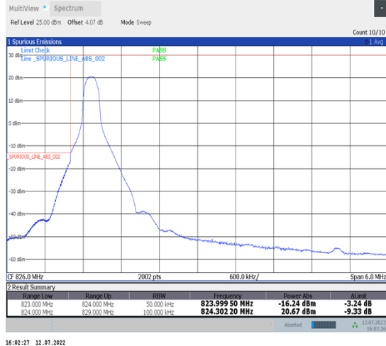
1-N26-824-849--15-5-L-1-DFT-PI2BPSK-Edge_1RB_Left-1@0-Ant1-seegraph-PASS-see graph
