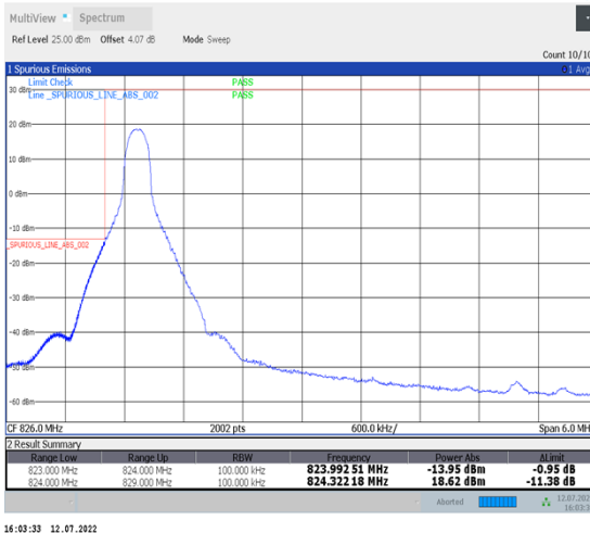
1-N26-824-849--15-5-L-4-CP-QPSK-Edge_1RB_Left-1@0-Ant1-seegraph-PASS-see graph
