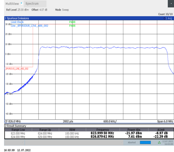
1-N26-824-849--15-5-L-3-DFT-PI2BPSK-Outer_Full-25@0-Ant1-seegraph-PASS-see graph
