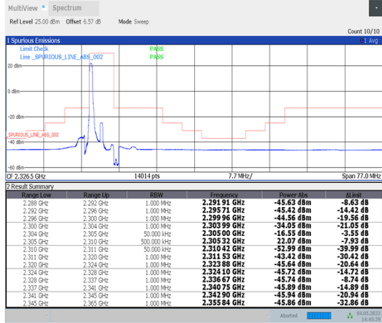
1-N30--15-5-L-1-DFT-PI2BPSK-Edge_1RB_Left-1@0-Ant1-PASS-see graph
