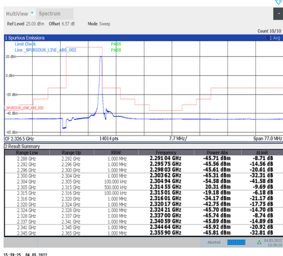
1-N30--15-10-H-5-CP-QPSK-Edge_1RB_Right-1@51-Ant1-PASS-see graph
