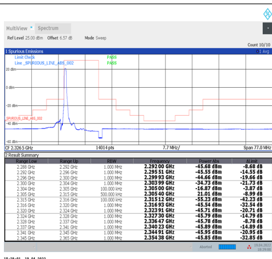
1-N30--30-10-L-1-DFT-PI2BPSK-Edge_1RB_Left-1@0-Ant1-PASS-see graph
