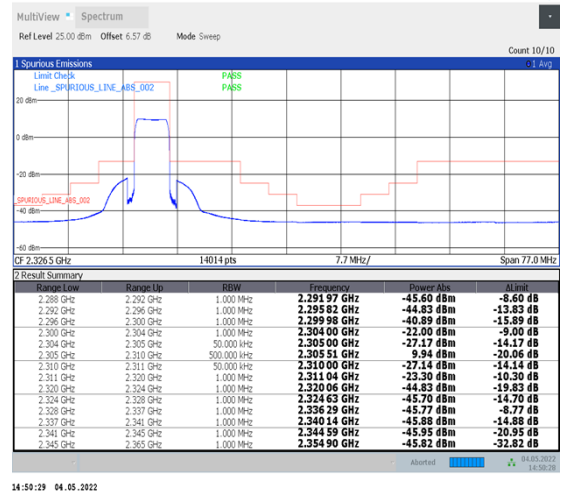
1-N30--15-5-L-6-CP-QPSK-Outer_Full-25@0-Ant1-PASS-see graph
