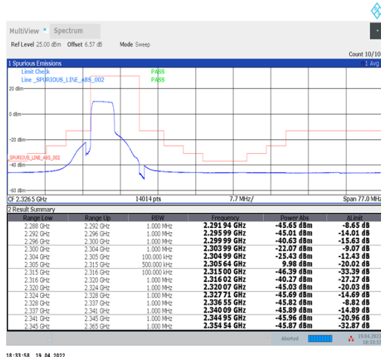
1-N30--30-10-L-6-CP-QPSK-Outer_Full-24@0-Ant1-PASS-see graph
