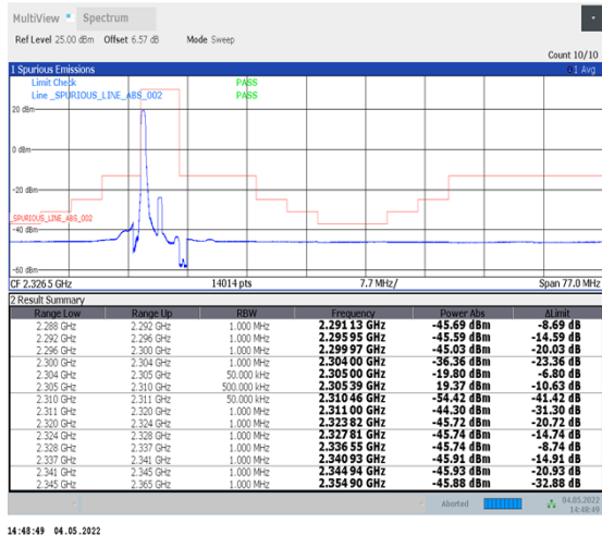
1-N30--15-5-L-4-CP-QPSK-Edge_1RB_Left-1@0-Ant1-PASS-see graph
