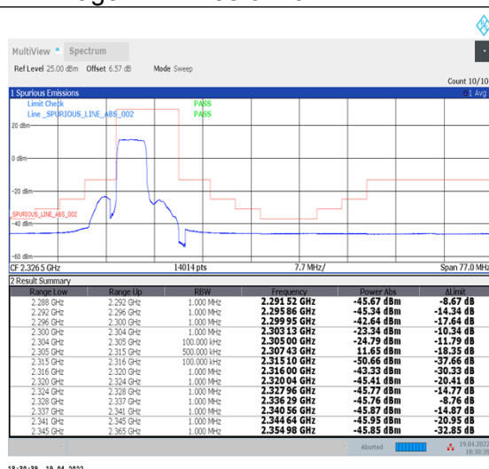
1-N30--30-10-L-3-DFT-PI2BPSK-Outer_Full-24@0-Ant1-PASS-see graph
