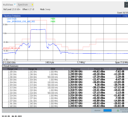
1-N30--15-10-H-3-DFT-PI2BPSK-Outer_Full-50@0-Ant1-PASS-see graph
