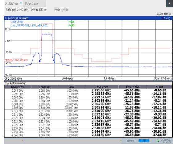
1-N30--15-5-L-3-DFT-PI2BPSK-Outer_Full-25@0-Ant1-PASS-see graph
