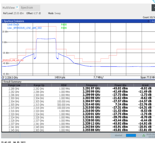
1-N30--15-10-H-6-CP-QPSK-Outer_Full-52@0-Ant1-PASS-see graph
