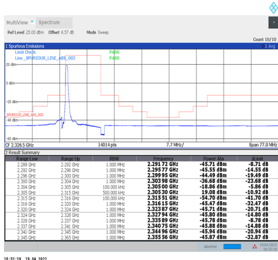
1-N30--30-10-L-4-CP-QPSK-Edge_1RB_Left-1@0-Ant1-PASS-see graph
