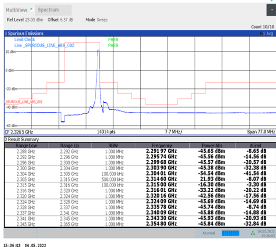
1-N30--15-10-H-2-DFT-PI2BPSK-Edge_1RB_Right-1@51-Ant1-PASS-see graph
