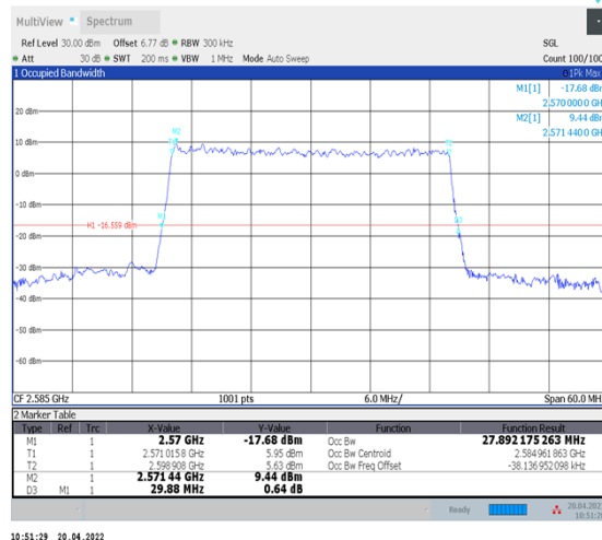
1-N38--30-30-L-9-CP-256QAM-Outer_Full-78@0- Ant1-27.892-29.880-≤30-PASS
