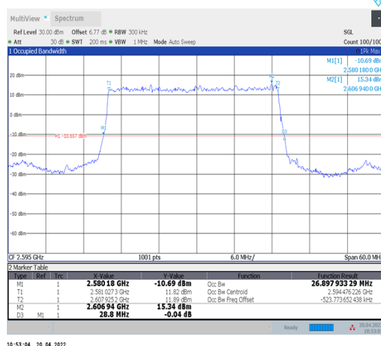
1-N38--30-30-M-2-DFT-PI2BPSK-Outer_Full-75@0- Ant1-26.898-28.800-≤30-PASS
