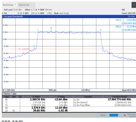
1-N38--30-30-L-8-CP-64QAM-Outer_Full-78@0- Ant1-27.905-30.660-≤30-PASS
