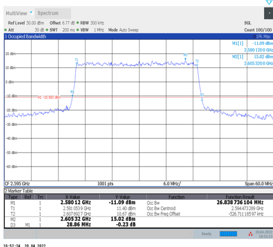
1-N38--30-30-M-1-DFT-QPSK-Outer_Full-75@0- Ant1-26.839-28.860-≤30-PASS
