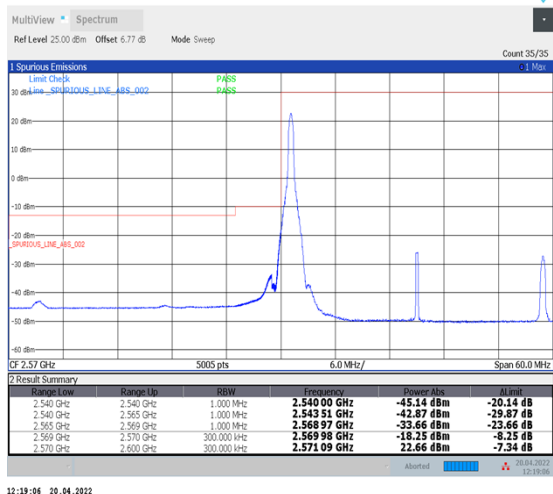
1-N38--30-30-L-1-DFT-PI2BPSK-Edge_1RB_Left-1@0-Ant1-PASS-see graph
