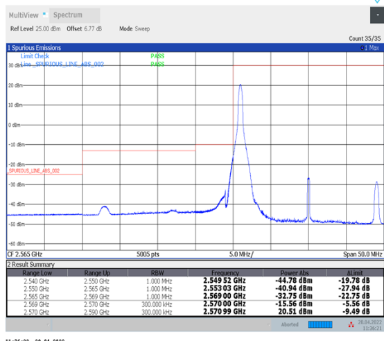
1-N38--30-20-L-4-CP-QPSK-Edge_1RB_Left-1@0-Ant1-PASS-see graph
