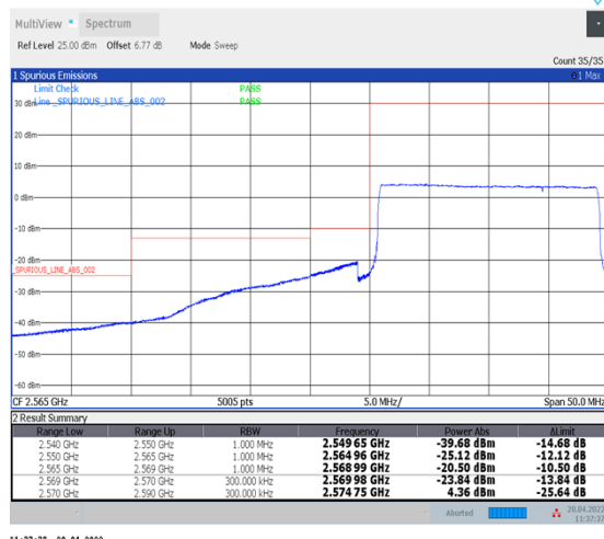
1-N38--30-20-L-6-CP-QPSK-Outer_Full-51@0-Ant1-PASS-see graph
