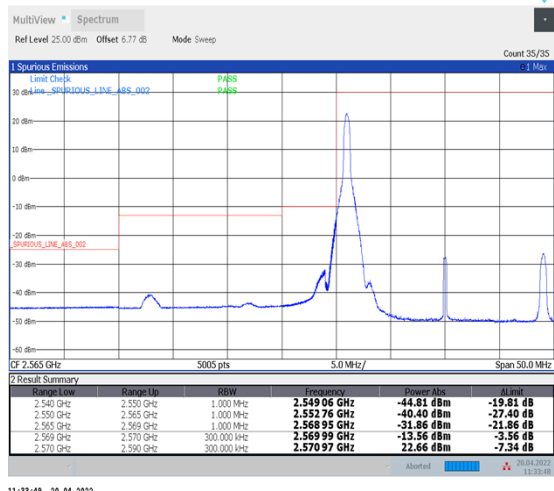
1-N38--30-20-L-1-DFT-PI2BPSK-Edge_1RB_Left-1@0-Ant1-PASS-see graph
