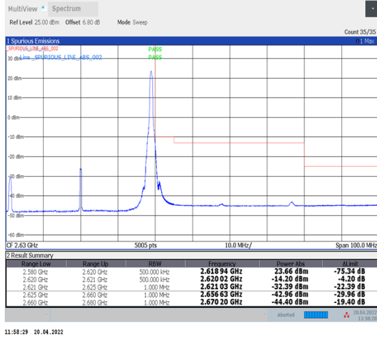
1-N38--30-40-H-2-DFT-PI2BPSK-Edge_1RB_Right-1@105-Ant1-PASS-see graph
