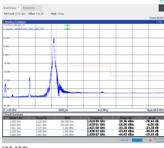
1-N38--30-20-H-5-CP-QPSK-Edge_1RB_Right-1@50-Ant1-PASS-see graph
