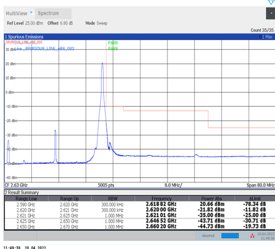
1-N38--30-30-H-5-CP-QPSK-Edge_1RB_Right-1@77-Ant1-PASS-see graph
