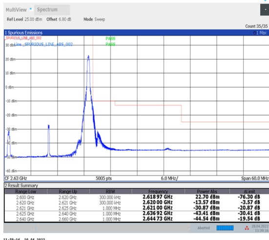
1-N38--30-20-H-2-DFT-PI2BPSK-Edge_1RB_Right-1@50-Ant1-PASS-see graph
