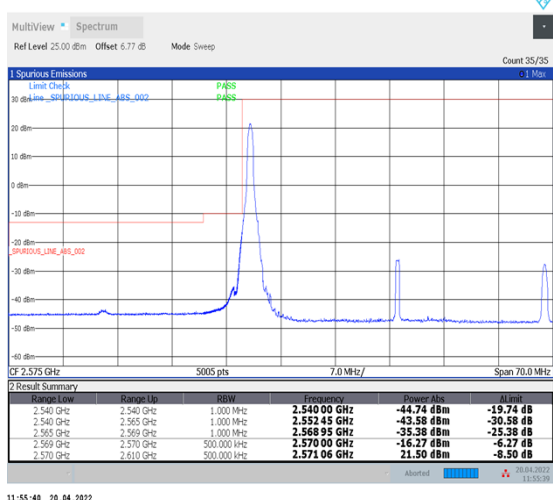
1-N38--30-40-L-4-CP-QPSK-Edge_1RB_Left-1@0-Ant1-PASS-see graph
