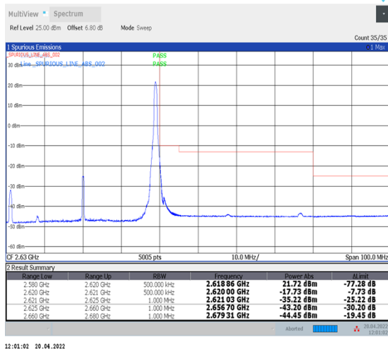
1-N38--30-40-H-5-CP-QPSK-Edge_1RB_Right-1@105-Ant1-PASS-see graph
