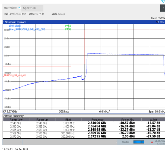
1-N38--30-30-L-6-CP-QPSK-Outer_Full-78@0-Ant1-PASS-see graph
