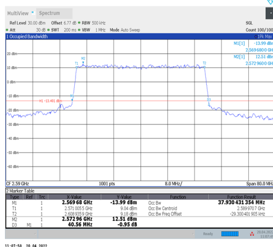
1-N38--30-40-L-8-CP-64QAM-Outer_Full-106@0-Ant1-37.93-40.560-≤40-PASS
