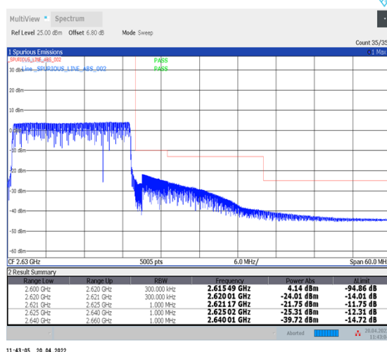
1-N38--30-20-H-6-CP-QPSK-Outer_Full-51@0-Ant1-PASS-see graph
