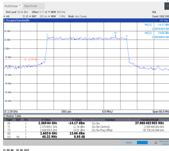
1-N38--30-40-L-6-CP-QPSK-Outer_Full-106@0-Ant1-37.96-40.320-≤40-PASS
