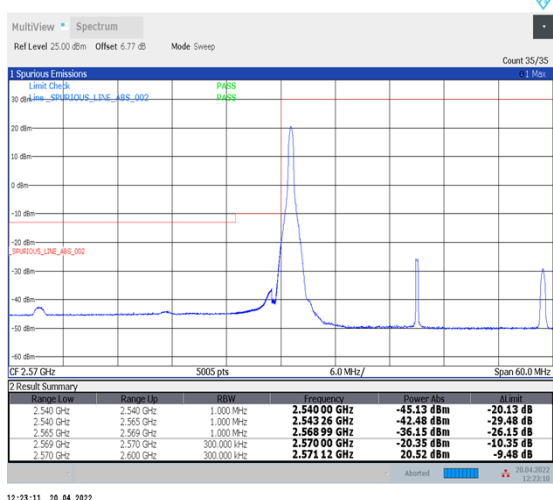
1-N38--30-30-L-4-CP-QPSK-Edge_1RB_Left-1@0-Ant1-PASS-see graph
