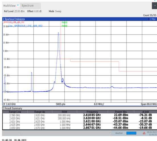
1-N38--30-30-H-2-DFT-PI2BPSK-Edge_1RB_Right-1@77-Ant1-PASS-see graph
