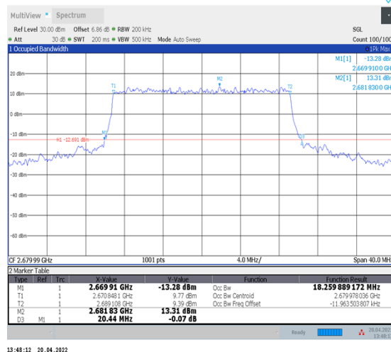
1-N41--30-20-H-8-CP-64QAM-Outer_Full-51@0- Ant1-18.26-20.440-≤20-PASS
