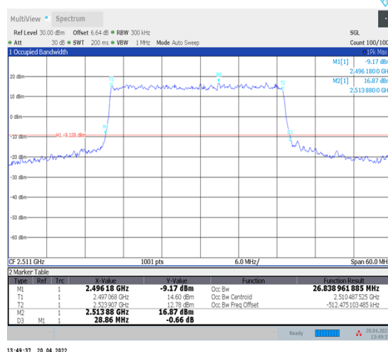
1-N41--30-30-L-1-DFT-QPSK-Outer_Full-75@0- Ant1-26.839-28.860-≤30-PASS
