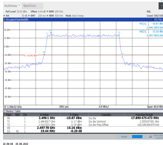
1-N41--30-20-L-4-DFT-64QAM-Outer_Full-50@0- Ant1-17.89-19.440-≤20-PASS
