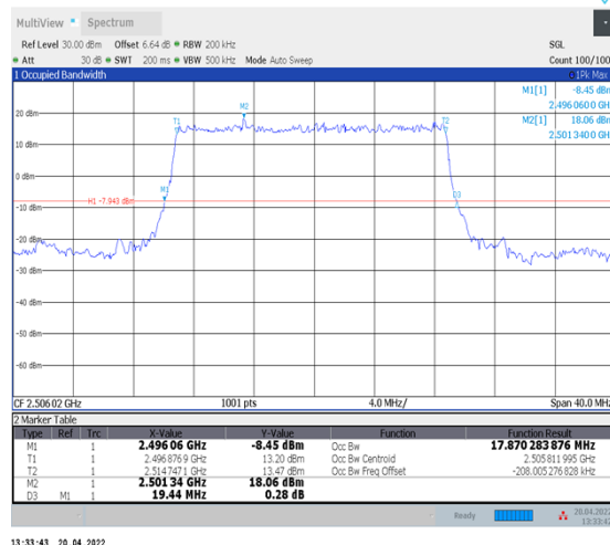
1-N41--30-20-L-2-DFT-PI2BPSK-Outer_Full-50@0- Ant1-17.87-19.440-≤20-PASS
