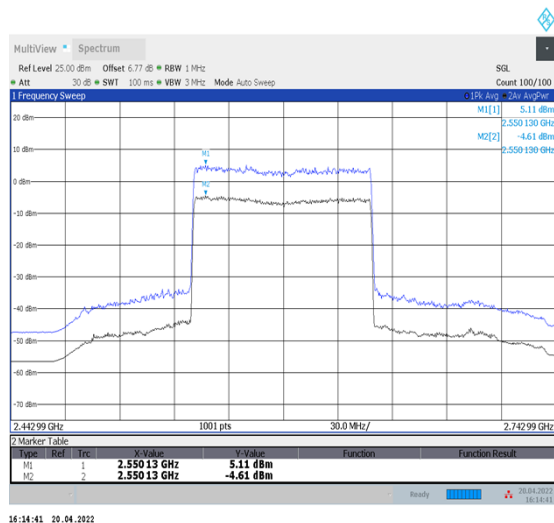
1-N41--30-100-M-1-DFT-256QAM-Outer_Full-270@0-Ant1-9.72-100%-0.00-9.72-PASS-≤13
