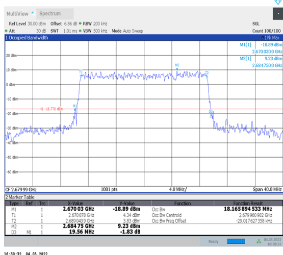
1-N41--30-20-H-9-CP-256QAM-Outer_Full-51@0- Ant1-18.166-19.560-≤20-PASS
