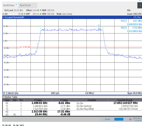
1-N41--30-20-L-1-DFT-QPSK-Outer_Full-50@0- Ant1-17.852-19.440-≤20-PASS
