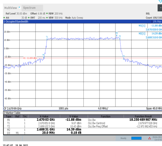
1-N41--30-20-H-6-CP-QPSK-Outer_Full-51@0-Ant1-18.25-20.000-≤20-PASS
