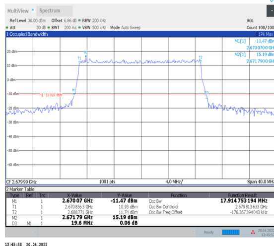
1-N41--30-20-H-4-DFT-64QAM-Outer_Full-50@0-Ant1-17.915-19.600-≤20-PASS
