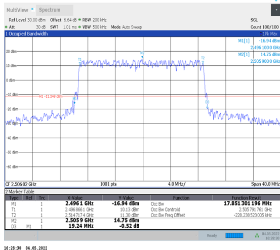
1-N41--30-20-L-3-DFT-16QAM-Outer_Full-50@0- Ant1-17.851-19.240-≤20-PASS
