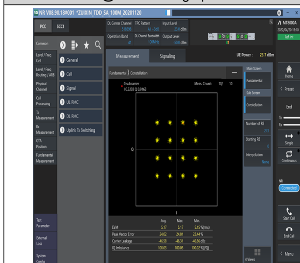
1-N41--30-100-M-7-CP-16QAM-Outer_Full-273@0-Ant1-see graph-PASS
