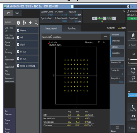
1-N41--30-100-M-8-CP-64QAM-Outer_Full-273@0-Ant1-see graph-PASS
