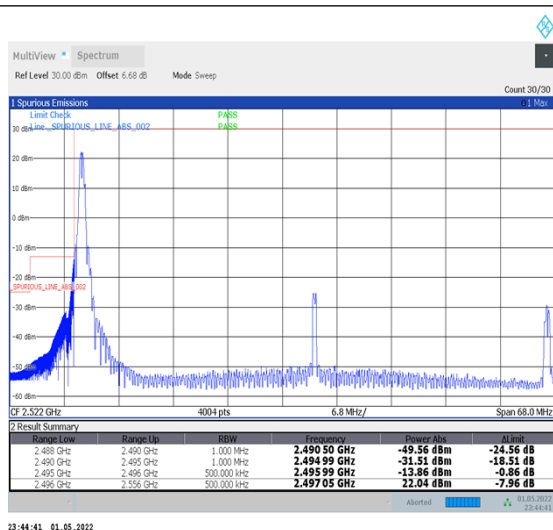
1-N41-PC2-30-60-L-4-CP-QPSK-Edge_1RB_Left-1@0-Ant2-PASS-see graph
