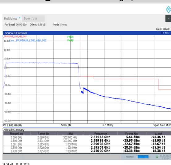
1-N41-PC2-30-30-H-6-CP-QPSK-Outer_Full-78@0-Ant2-PASS-see graph
