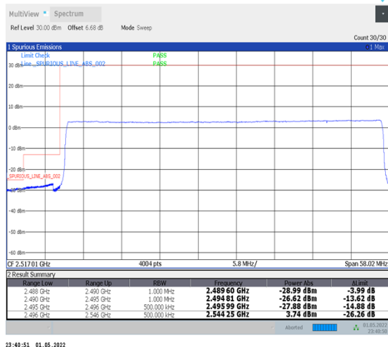
1-N41-PC2-30-50-L-6-CP-QPSK-Outer_Full-133@0-Ant2-PASS-see graph
