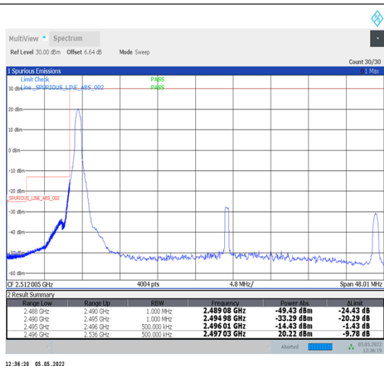
1-N41-PC2-30-40-L-4-CP-QPSK-Edge_1RB_Left-1@0-Ant2-PASS-see graph
