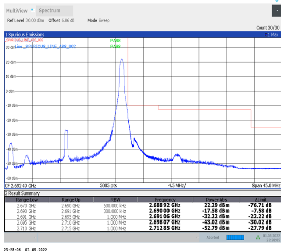
1-N41-PC2-30-20-H-5-CP-QPSK-Edge_1RB_Right-1@50-Ant2-PASS-see graph
