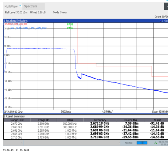
1-N41-PC2-30-20-H-6-CP-QPSK-Outer_Full-51@0-Ant2-PASS-see graph
