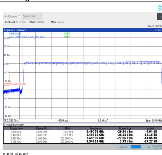
1-N41-PC2-30-60-L-6-CP-QPSK-Outer_Full-162@0-Ant2-PASS-see graph
