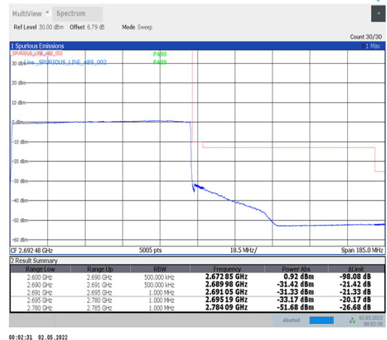
1-N41-PC2-30-90-H-6-CP-QPSK-Outer_Full-245@0-Ant2-PASS-see graph
