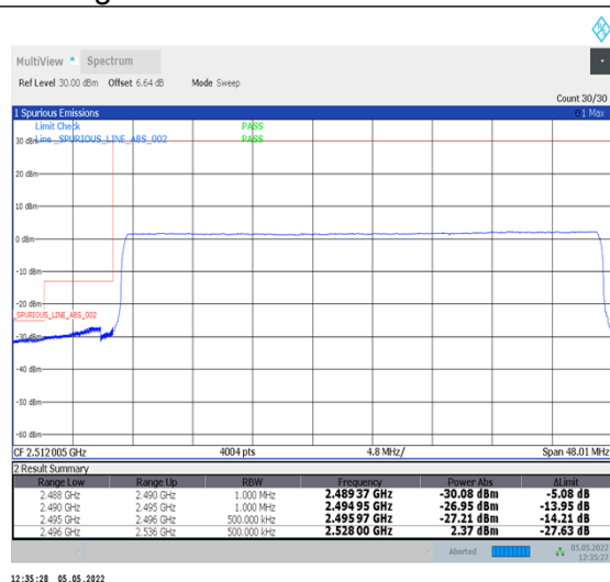
1-N41-PC2-30-40-L-6-CP-QPSK-Outer_Full-106@0-Ant2-PASS-see graph
