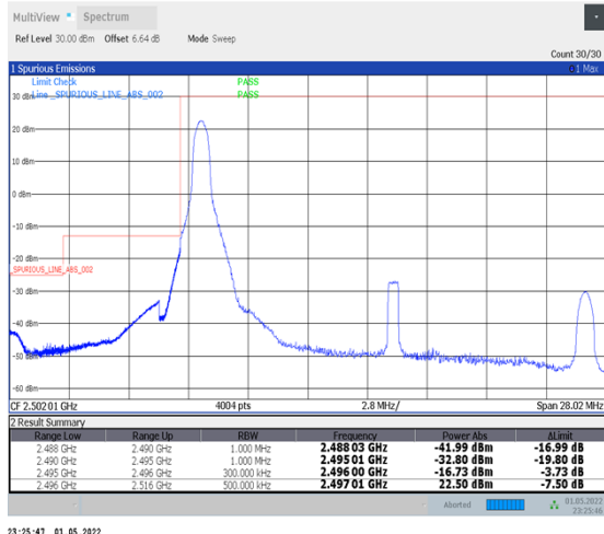
1-N41-PC2-30-20-L-4-CP-QPSK-Edge_1RB_Left-1@0-Ant2-PASS-see graph
