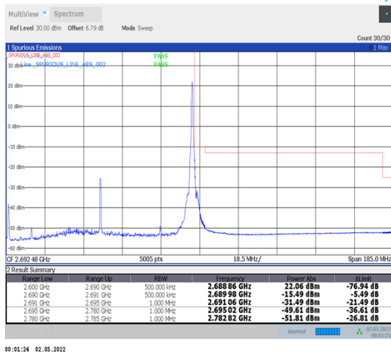
1-N41-PC2-30-90-H-5-CP-QPSK-Edge_1RB_Right-1@244-Ant2-PASS-see graph
