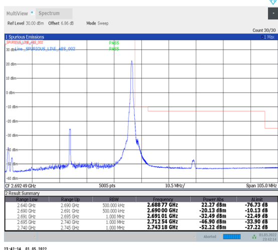
1-N41-PC2-30-50-H-5-CP-QPSK-Edge_1RB_Right-1@132-Ant2-PASS-see graph
