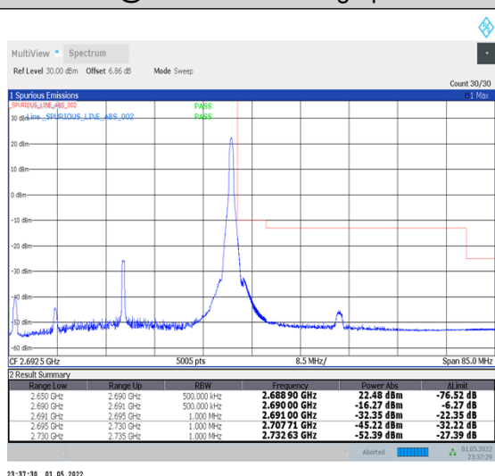
1-N41-PC2-30-40-H-5-CP-QPSK-Edge_1RB_Right-1@105-Ant2-PASS-see graph
