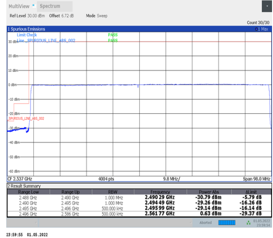
1-N41-PC2-30-90-L-6-CP-QPSK-Outer_Full-245@0-Ant2-PASS-see graph
