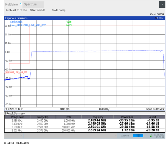
1-N41-PC2-30-70-L-6-CP-QPSK-Outer_Full-189@0-Ant2-PASS-see graph
