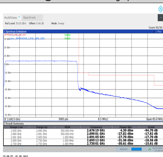
1-N41-PC2-30-40-H-6-CP-QPSK-Outer_Full-106@0-Ant2-PASS-see graph
