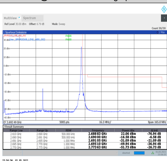
1-N41-PC2-30-80-H-5-CP-QPSK-Edge_1RB_Right-1@216-Ant2-PASS-see graph
