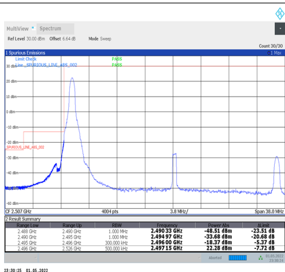
1-N41-PC2-30-30-L-4-CP-QPSK-Edge_1RB_Left-1@0-Ant2-PASS-see graph
