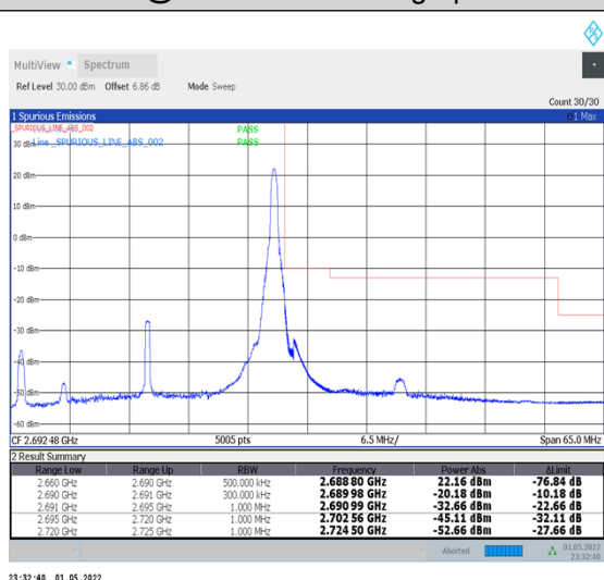
1-N41-PC2-30-30-H-5-CP-QPSK-Edge_1RB_Right-1@77-Ant2-PASS-see graph
