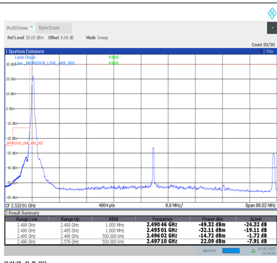
1-N41-PC2-30-80-L-4-CP-QPSK-Edge_1RB_Left-1@0-Ant2-PASS-see graph
