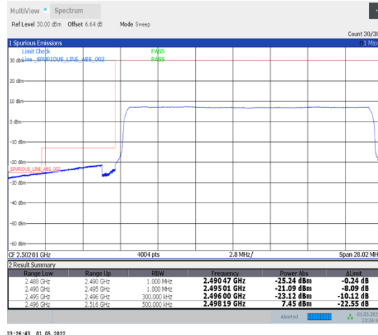
1-N41-PC2-30-20-L-6-CP-QPSK-Outer_Full-51@0-Ant2-PASS-see graph
