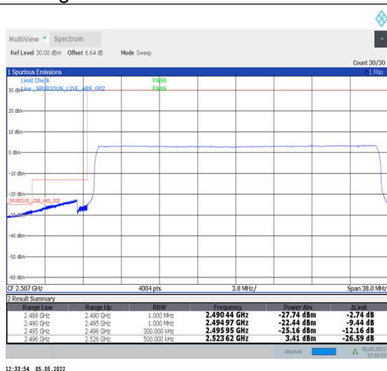
1-N41-PC2-30-30-L-6-CP-QPSK-Outer_Full-78@0-Ant2-PASS-see graph
