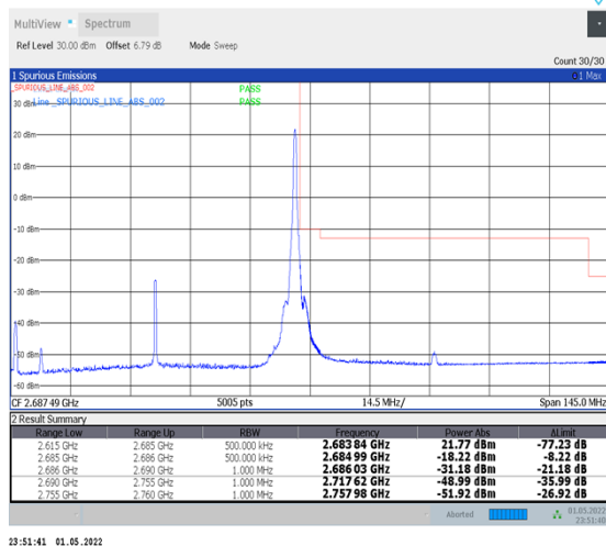
1-N41-PC2-30-70-H-5-CP-QPSK-Edge_1RB_Right-1@188-Ant2-PASS-see graph
