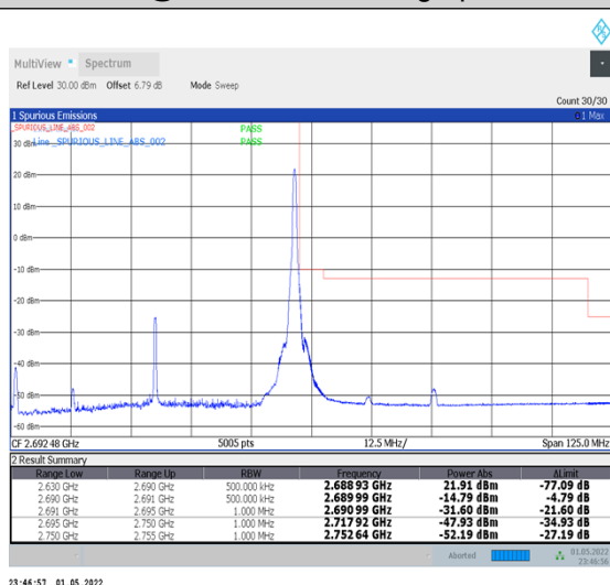
1-N41-PC2-30-60-H-5-CP-QPSK-Edge_1RB_Right-1@161-Ant2-PASS-see graph
