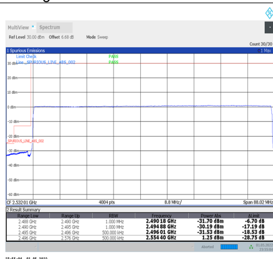
1-N41-PC2-30-80-L-6-CP-QPSK-Outer_Full-217@0-Ant2-PASS-see graph
