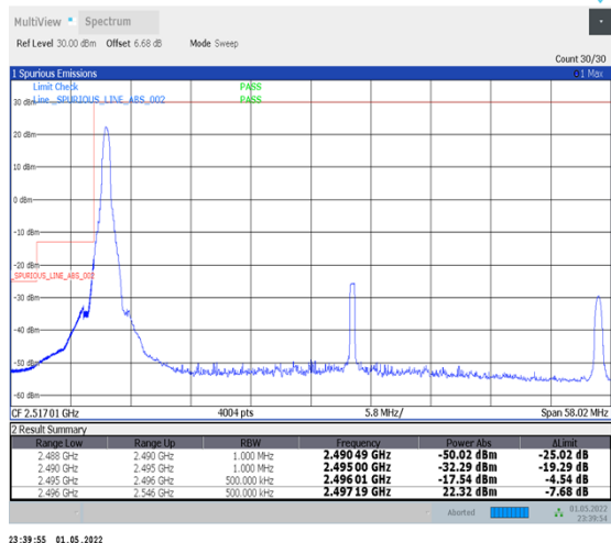
1-N41-PC2-30-50-L-4-CP-QPSK-Edge_1RB_Left-1@0-Ant2-PASS-see graph
