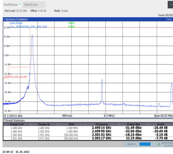
1-N41-PC2-30-70-L-4-CP-QPSK-Edge_1RB_Left-1@0-Ant2-PASS-see graph
