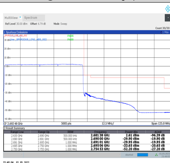
1-N41-PC2-30-60-H-6-CP-QPSK-Outer_Full-162@0-Ant2-PASS-see graph
