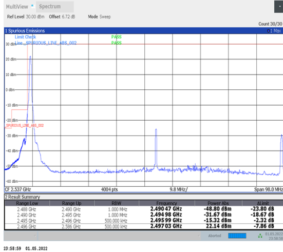
1-N41-PC2-30-90-L-4-CP-QPSK-Edge_1RB_Left-1@0-Ant2-PASS-see graph
