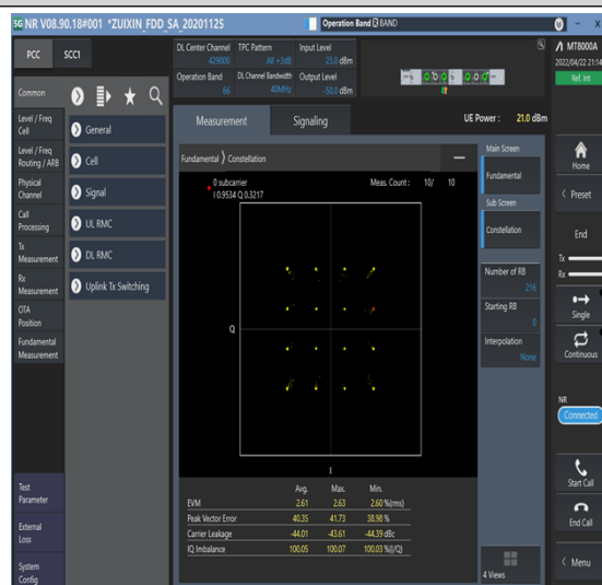
1-N66-PC3-15-40-M-3-DFT-16QAM-Outer_Full-216@0-Ant1-see graph-PASS
