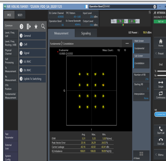
1-N66-PC3-15-40-M-7-CP-16QAM-Outer_Full-216@0-Ant1-see graph-PASS
