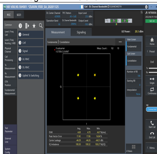
1-N66-PC3-15-20-M-6-CP-QPSK-Outer_Full-106@0-Ant1-see graph-PASS
