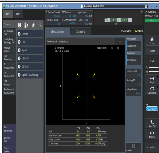
1-N66-PC3-15-40-M-2-DFT-QPSK-Outer_Full-216@0-Ant1-see graph-PASS
