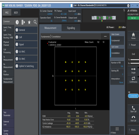
1-N66-PC3-15-20-M-7-CP-16QAM-Outer_Full-106@0-Ant1-see graph-PASS
