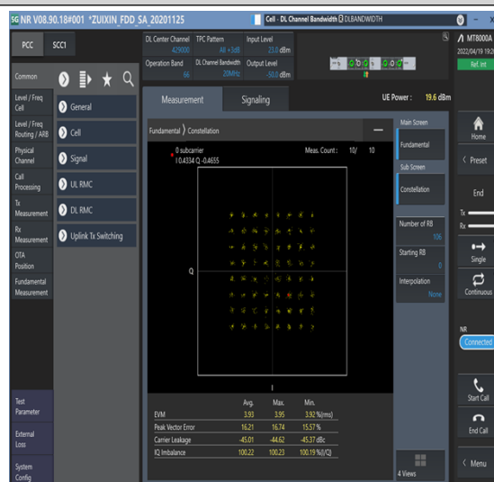
1-N66-PC3-15-20-M-8-CP-64QAM-Outer_Full-106@0-Ant1-see graph-PASS
