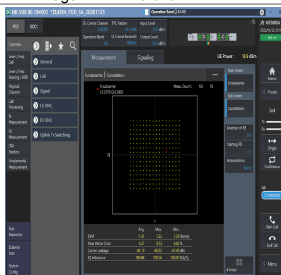
1-N66-PC3-15-40-M-9-CP-256QAM-Outer_Full-216@0-Ant1-see graph-PASS
