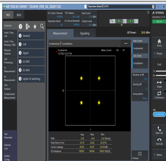
1-N66-PC3-15-40-M-6-CP-QPSK-Outer_Full-216@0-Ant1-see graph-PASS
