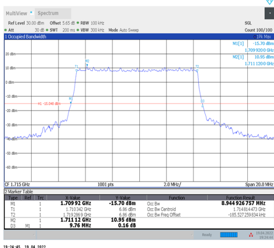
1-N66-PC3-15-10-L-4-DFT-64QAM-Outer_Full-50@0-Ant1-8.945-9.760-≤10-PASS
