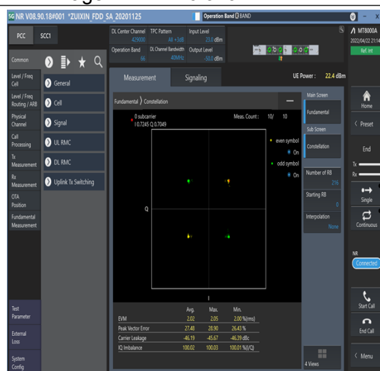
1-N66-PC3-15-40-M-1-DFT-PI2BPSK-Outer_Full-216@0-Ant1-see graph-PASS
