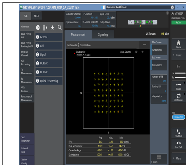
1-N66-PC3-15-40-M-8-CP-64QAM-Outer_Full-216@0-Ant1-see graph-PASS
