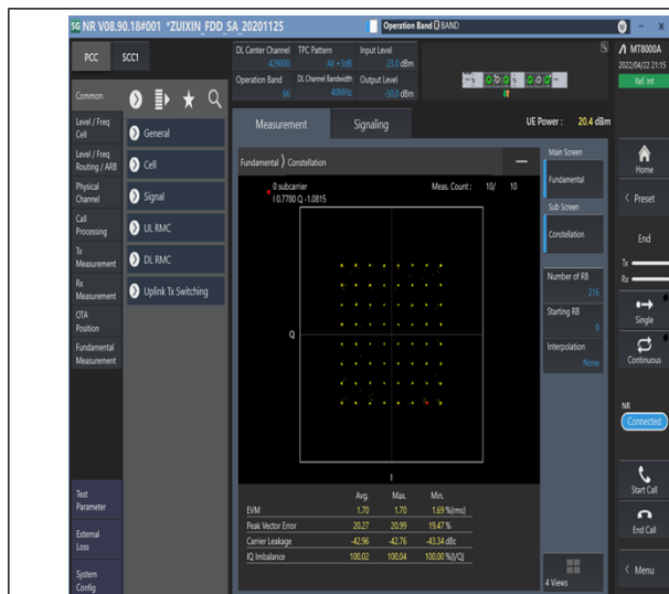
1-N66-PC3-15-40-M-4-DFT-64QAM-Outer_Full-216@0-Ant1-see graph-PASS
