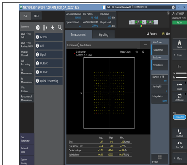
1-N66-PC3-15-20-M-9-CP-256QAM-Outer_Full-106@0-Ant1-see graph-PASS
