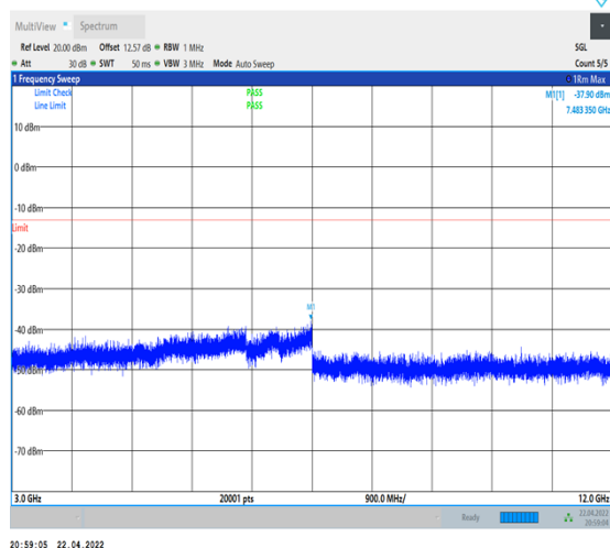
1-N66-PC3-15-40-L-1-DFT-PI2BPSK- Inner_1RB_Left-1@1-3000-12000-Ant1--37.90--13- PASS
