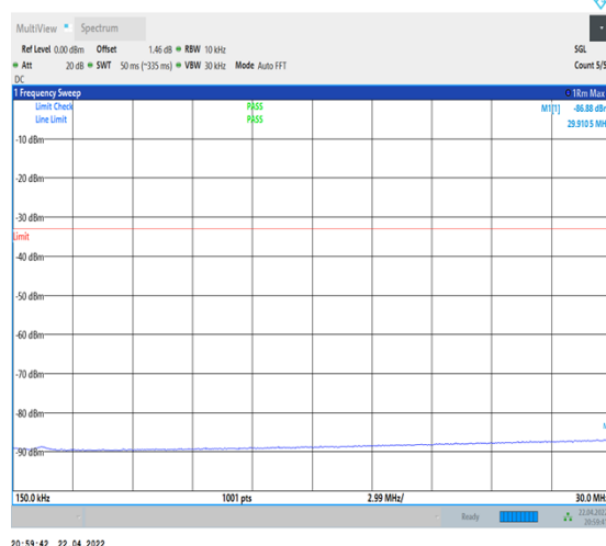
1-N66-PC3-15-40-M-1-DFT-PI2BPSK- Inner_1RB_Left-1@1-0.15-30-Ant1--86.88--33-PASS
