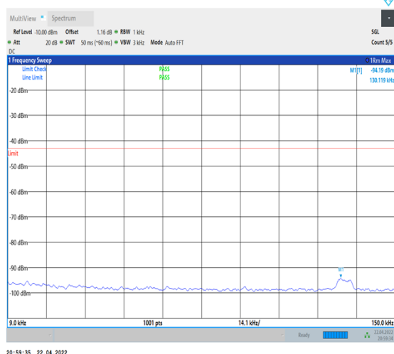
1-N66-PC3-15-40-M-1-DFT-PI2BPSK- Inner_1RB_Left-1@1-0.009-0.15-Ant1--94.19--43- PASS
