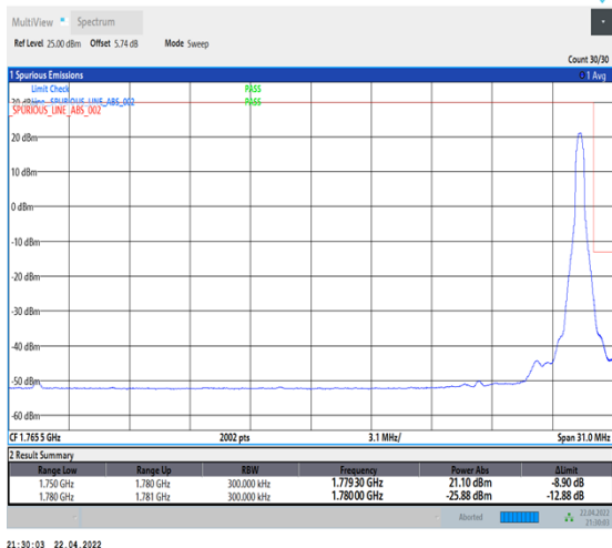
1-N66-PC3-15-30-H-2-DFT-PI2BPSK-Edge_1RB_Right-1@159-Ant1-seegraph-PASS-see graph
