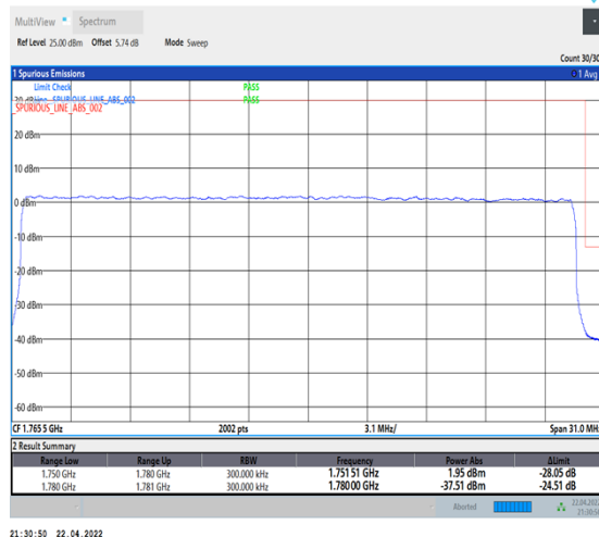
1-N66-PC3-15-30-H-3-DFT-PI2BPSK-Outer_Full-160@0-Ant1-seegraph-PASS-see graph
