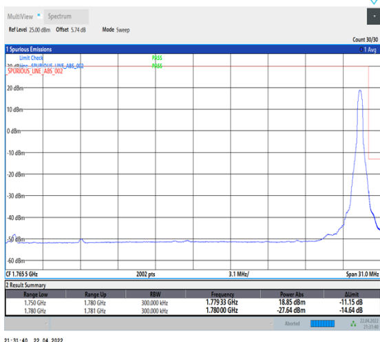
1-N66-PC3-15-30-H-5-CP-QPSK-Edge_1RB_Right-1@159-Ant1-seegraph-PASS-see graph
