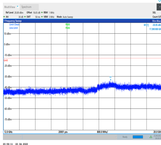
1-N66-PC3-15-40-L-1-DFT-PI2BPSK- Inner_1RB_Left-1@1-12000-20000-Ant1--33.95--13- PASS
