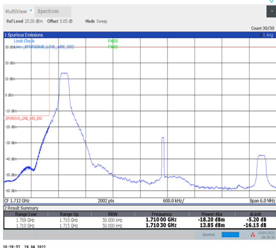
1-N66-PC3-15-5-L-4-CP-QPSK-Edge_1RB_Left-1@0-Ant1-seegraph-PASS-see graph
