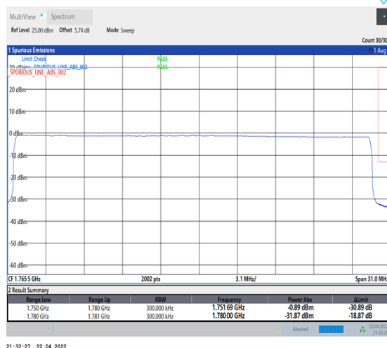
1-N66-PC3-15-30-H-6-CP-QPSK-Outer_Full-160@0-Ant1-seegraph-PASS-see graph
