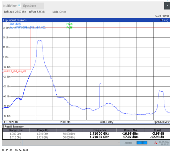
1-N66-PC3-15-5-L-1-DFT-PI2BPSK-Edge_1RB_Left-1@0-Ant1-seegraph-PASS-see graph
