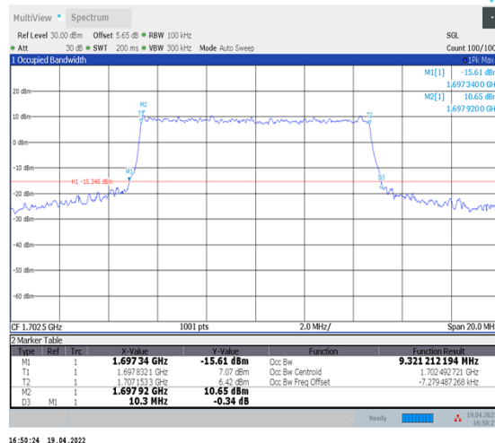
1-N70--15-10-M-6-CP-QPSK-Outer_Full-52@0-Ant1-9.321-10.300-≤10-PASS
