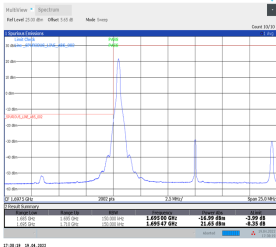
1-N70--15-15-L-1-DFT-PI2BPSK-Edge_1RB_Left-1@0-Ant1-seegraph-PASS-see graph
