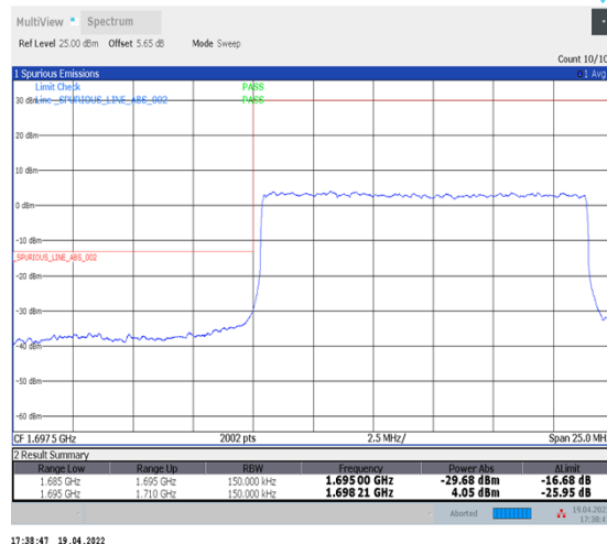
1-N70--15-15-L-3-DFT-PI2BPSK-Outer_Full-75@0-Ant1-seegraph-PASS-see graph
