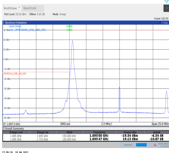
1-N70--15-15-L-4-CP-QPSK-Edge_1RB_Left-1@0-Ant1-seegraph-PASS-see graph
