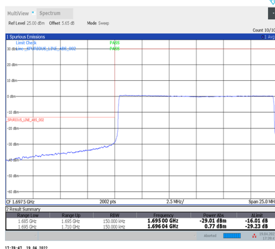
1-N70--15-15-L-6-CP-QPSK-Outer_Full-79@0-Ant1-seegraph-PASS-see graph
