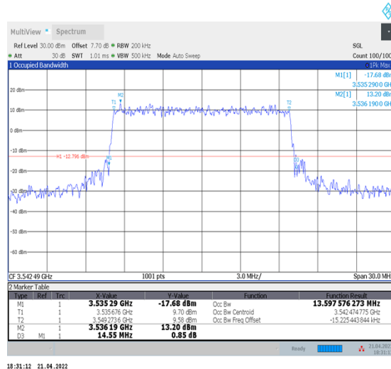
1-N78-3450-3550--30-15-H-7-CP-16QAM-Outer_Full-38@0-Ant1-13.598-14.550-≤15-PASS
