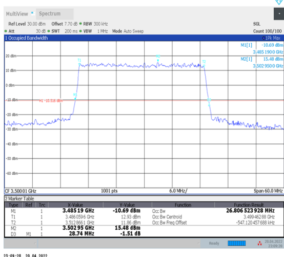
1-N78-3450-3550--30-30-M-1-DFT-QPSK-Outer_Full-75@0-Ant1-26.807-28.740-≤30-PASS
