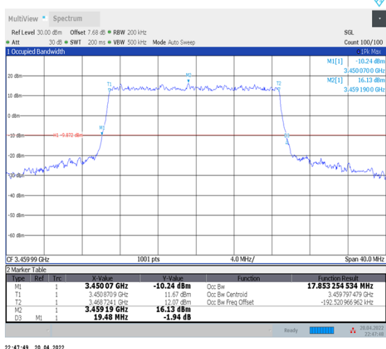
1-N78-3450-3550--30-20-L-1-DFT-QPSK-Outer_Full-50@0-Ant1-17.853-19.480-≤20-PASS
