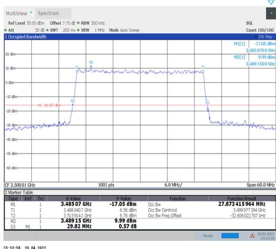
1-N78-3450-3550--30-30-M-9-CP-256QAM-Outer_Full-78@0-Ant1-27.873-29.820-≤30-PASS
