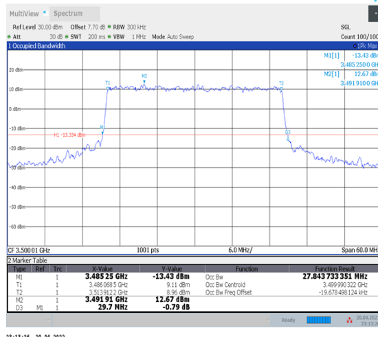
1-N78-3450-3550--30-30-M-8-CP-64QAM-Outer_Full-78@0-Ant1-27.844-29.700-≤30-PASS
