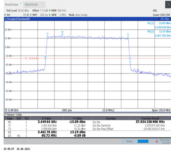
1-N78-3450-3550--30-60-L-4-DFT-64QAM-Outer_Full-162@0-Ant1-57.934-60.720-≤60-PASS
