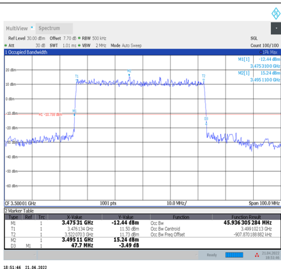
1-N78-3450-3550--30-50-M-1-DFT-QPSK-Outer_Full-128@0-Ant1-45.936-47.700-≤50-PASS
