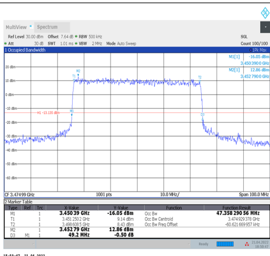
1-N78-3450-3550--30-50-L-6-CP-QPSK-Outer_Full-133@0-Ant1-47.358-49.200-≤50-PASS
