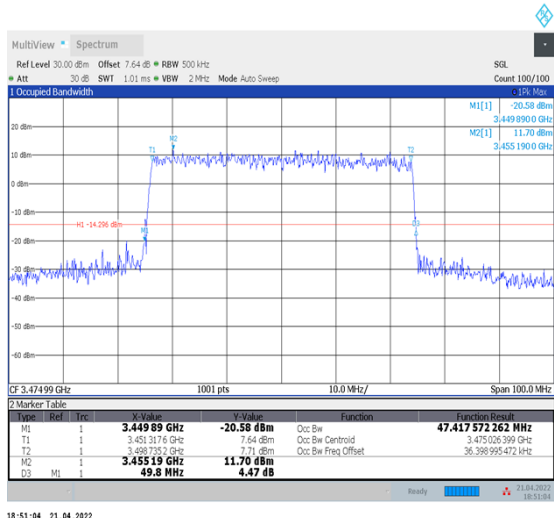
1-N78-3450-3550--30-50-L-8-CP-64QAM-Outer_Full-133@0-Ant1-47.418-49.800-≤50-PASS
